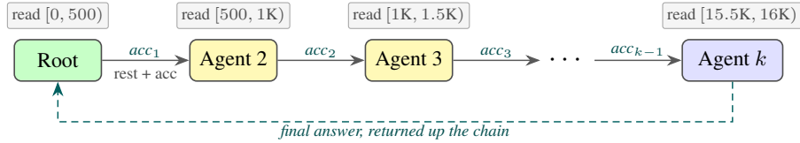
(b) Sequential fold , for order-dependent tasks (variable tracking, running state). Each agent reads the next slice, updates the accumulator, and delegates the rest of the document to the next agent.
