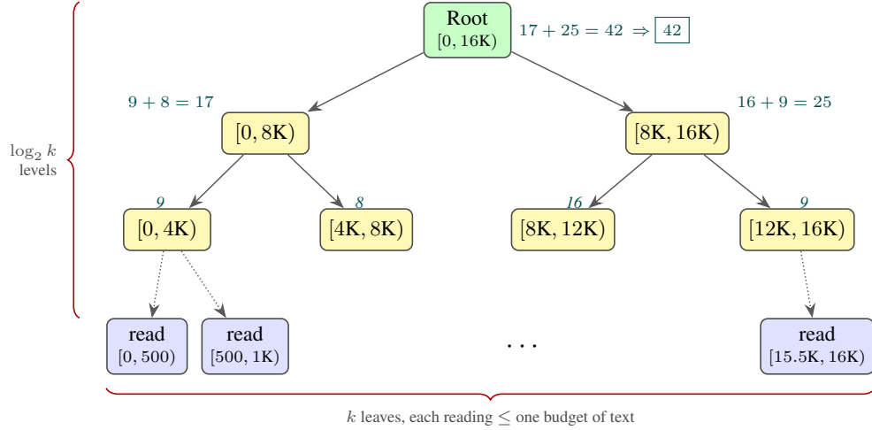
(a) Tree reduce , for order-independent tasks (counting, frequency, retrieval). Internal nodes and the root delegate half their range to subagents. Leaves read one chunk and compute a leaf op which is aggregated up the tree. Root determines the final answer.
