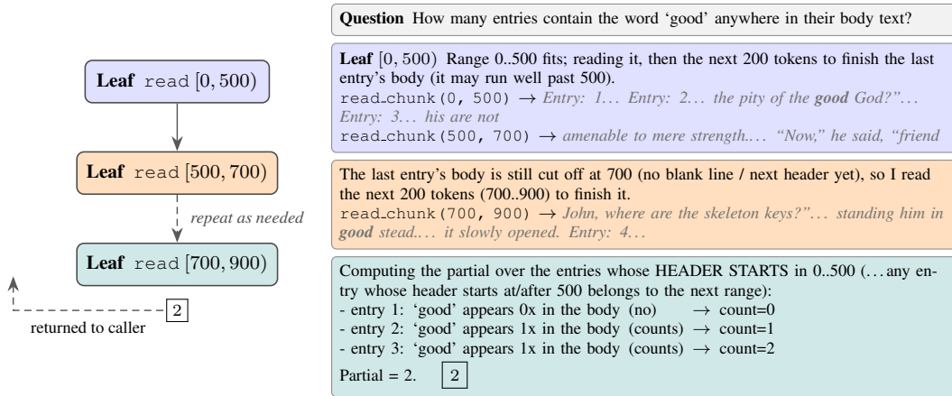
Figure 3: Boundary handling . A leaf/fold agent owns the records that start in its range. It reads 200 additional tokens at a time until its last record is complete.
