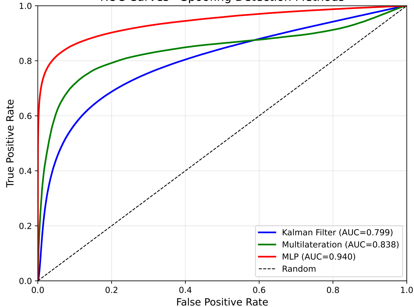
ROC Curves - Spoofing Detection Methods
