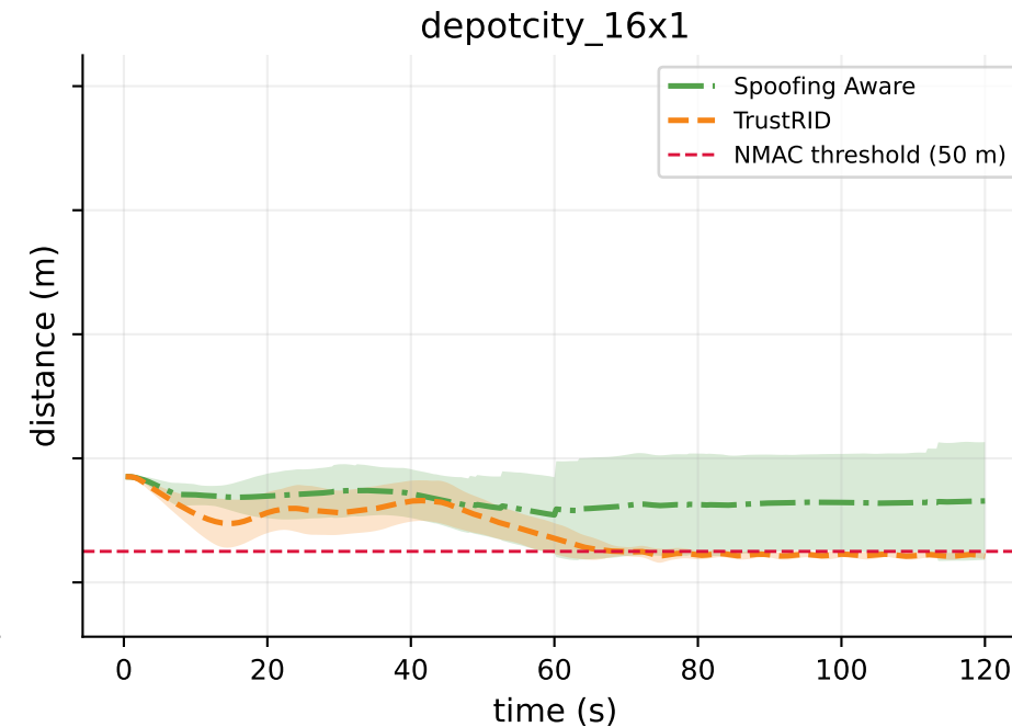
Min Benign-Spoofers Distance Through Time (mean \pm std, by Scenario) Note: benign hosts are excluded from this metric after reaching goal.
