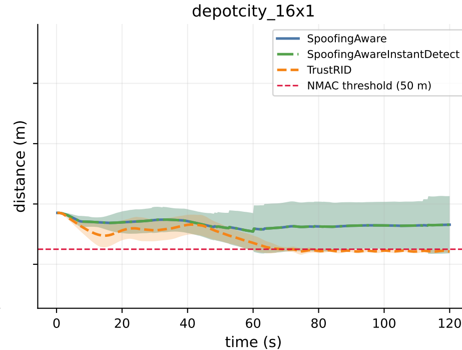
Min Benign-Spoofing Distance Through Time (mean \pm std, by Scenario)
