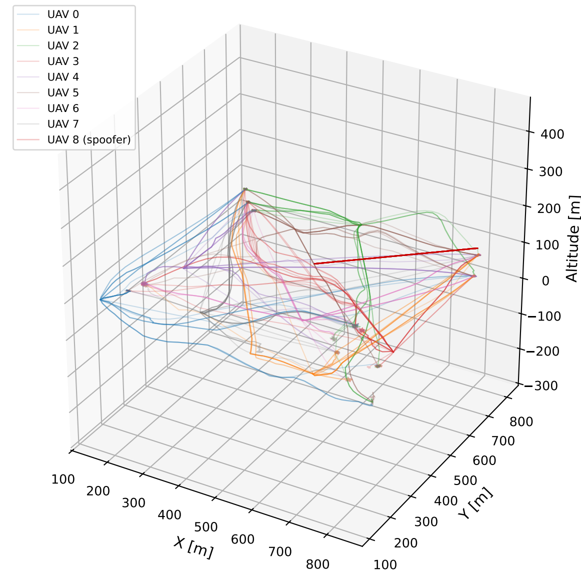
TrustRID (runs=30)
