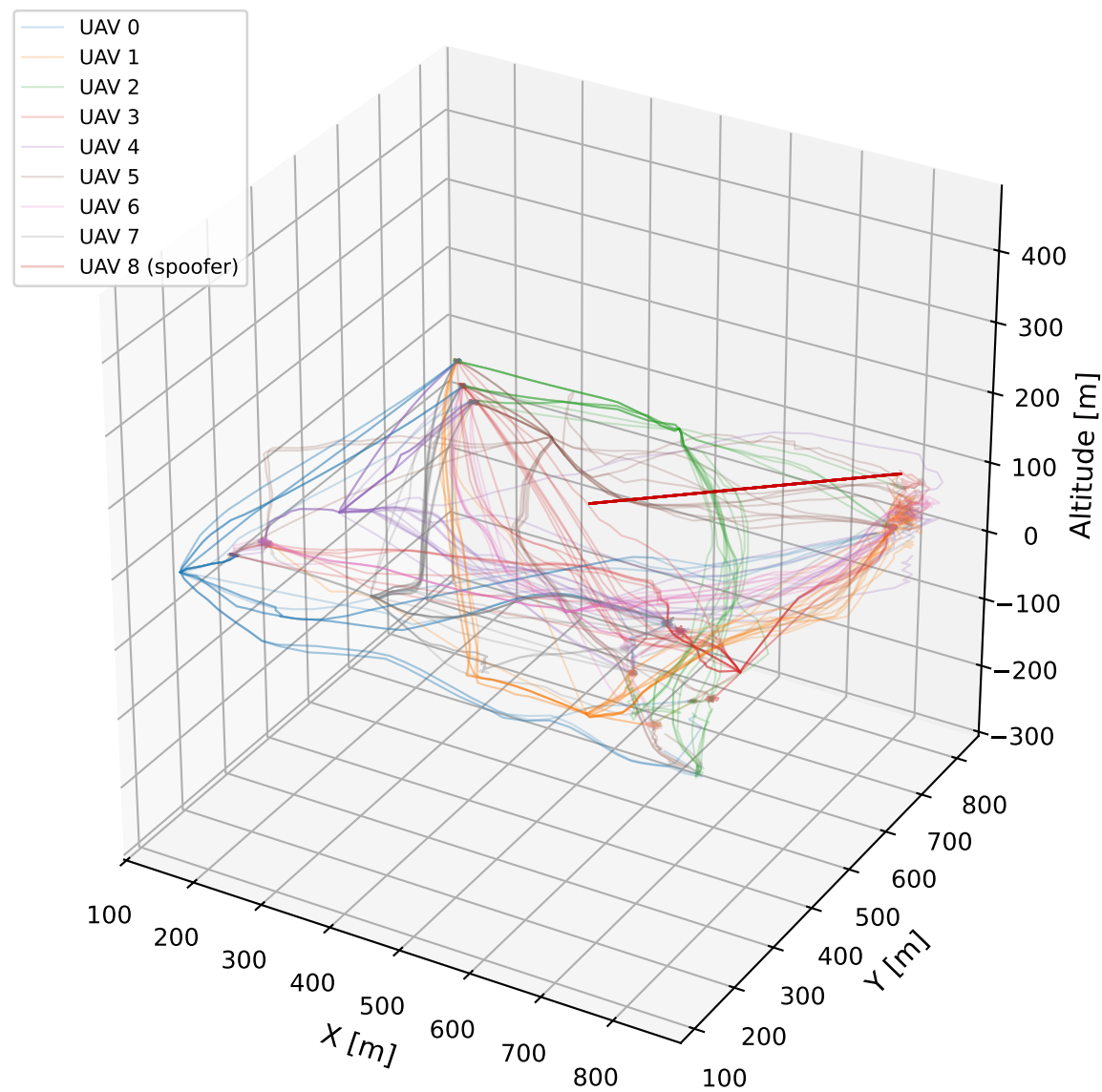
SpoofingAware (runs=30)
