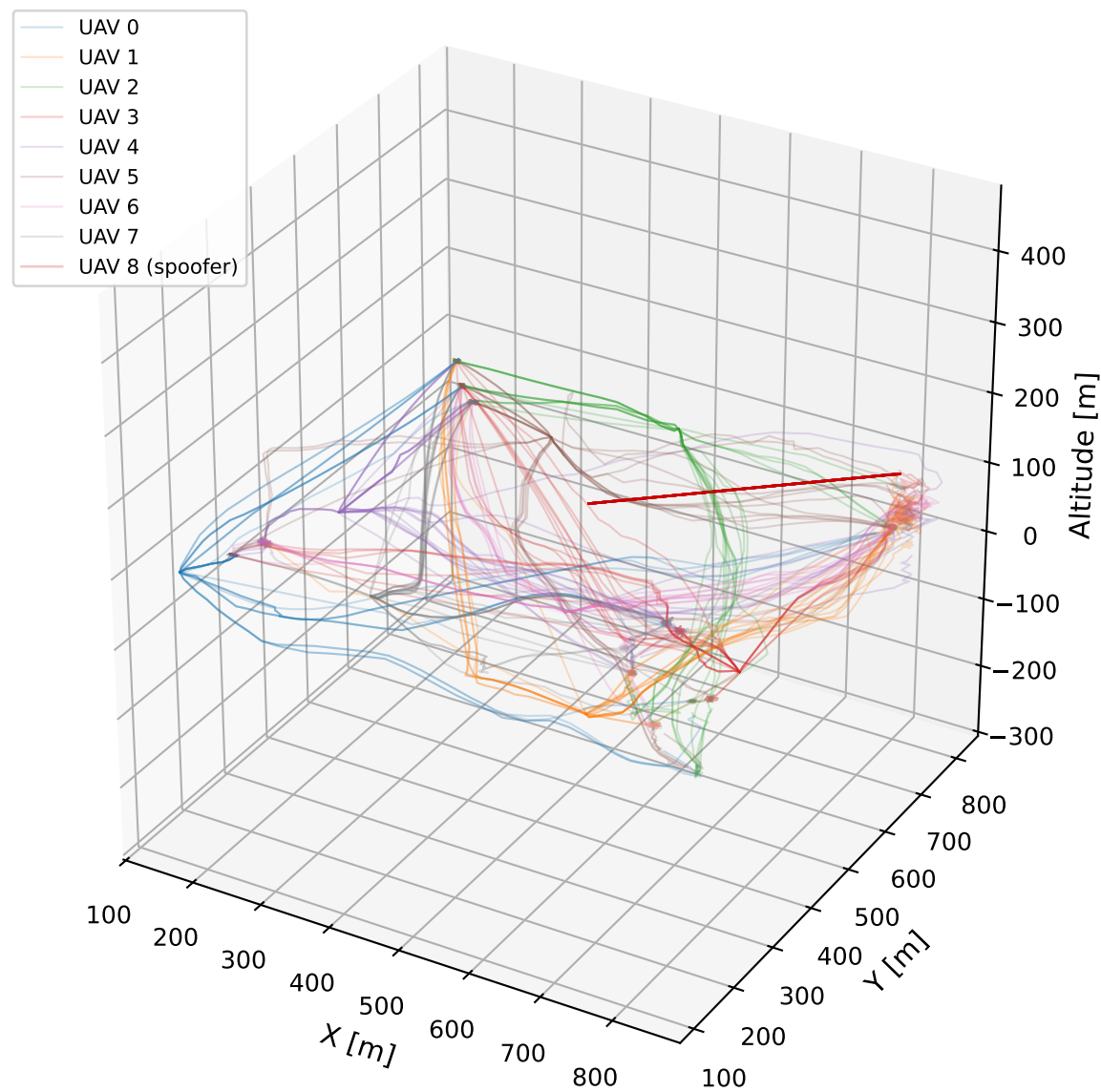
SpoofingAwareInstantDetect (runs=30)
