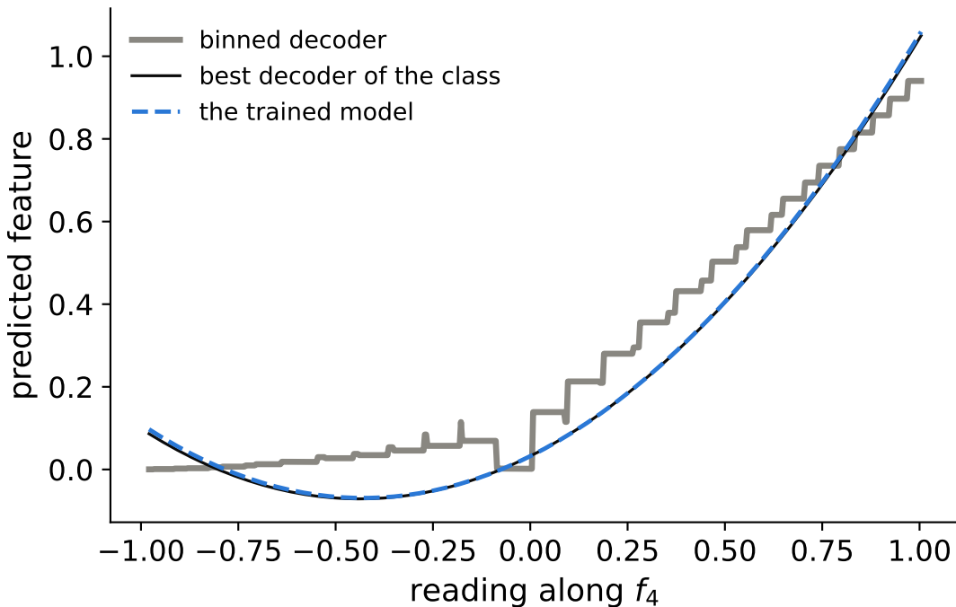
single bilinear MLP, seed 10: \hat{x}_4 along the line of f_4
