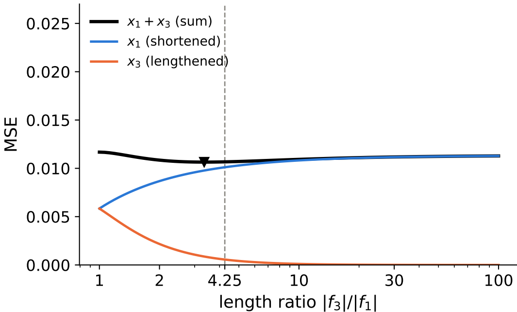
closed-form decoder
