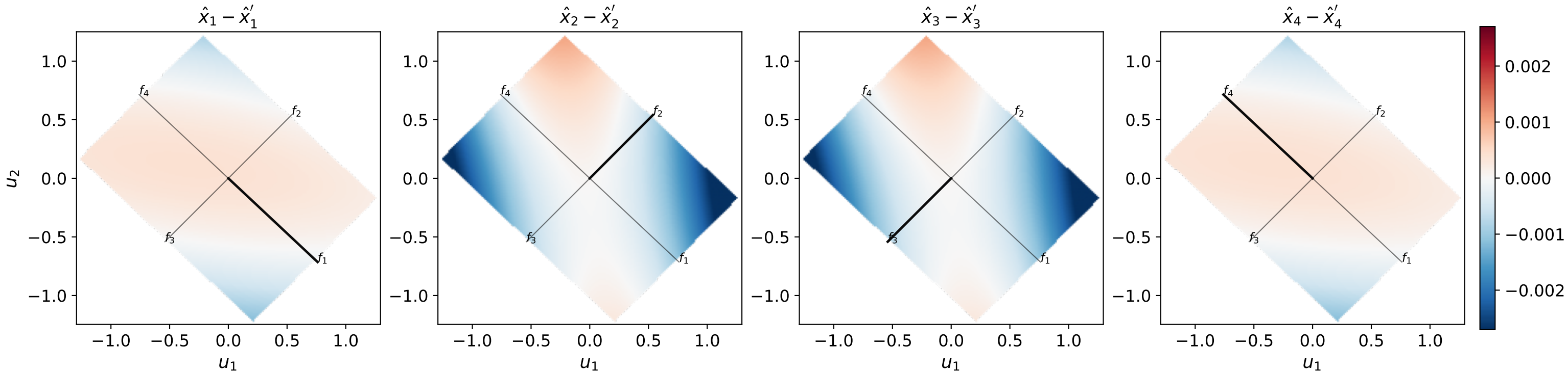
model – best decoder of the class, single bilinear MLP, seed 10
