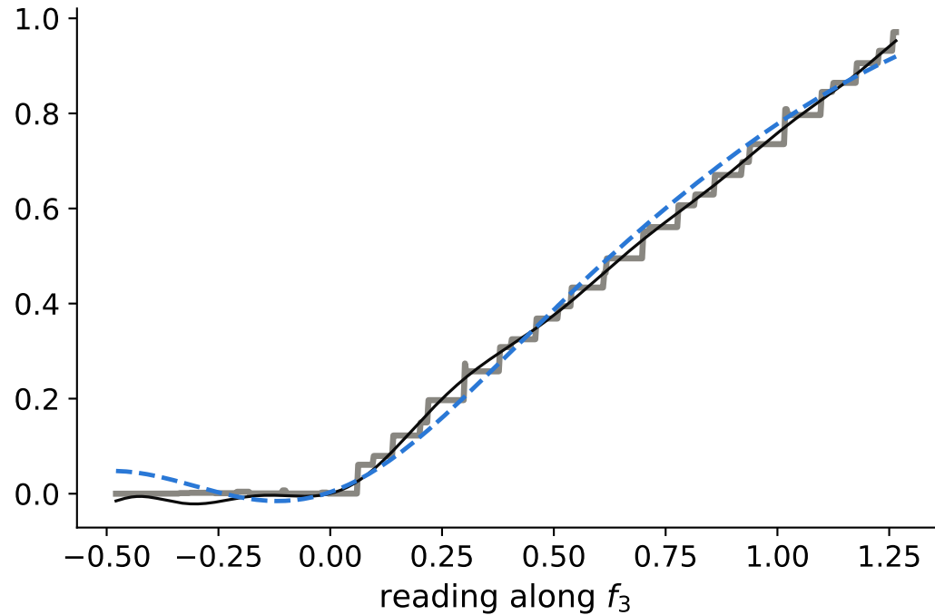
four bilinear MLPs, seed 9: \hat{x}_3 along the line of f_3
