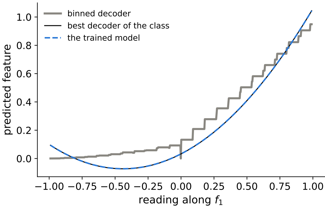
single bilinear MLP, seed 10: \hat{x}_1 along the line of f_1
