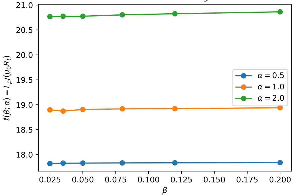
Inductance scaling
