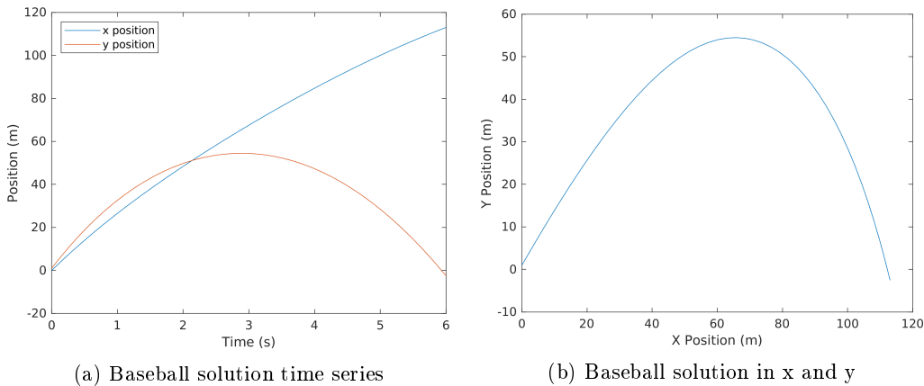
Figure 13.4: Simulated flight of a baseball including drag force including drag force
