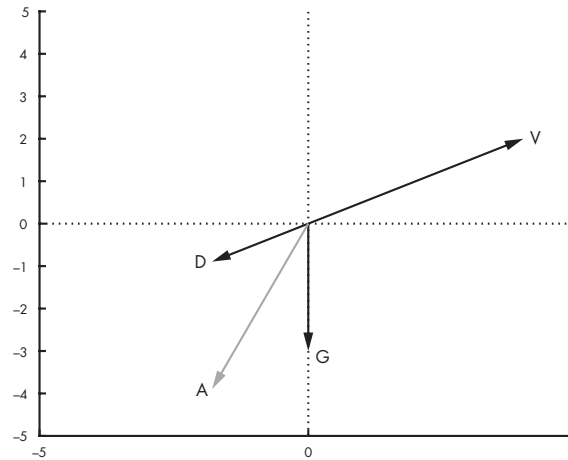
Figure 13.3: Diagram of velocity, \mathbf{V} ; acceleration due to drag force, \mathbf{D} ; acceleration due to gravity, \mathbf{G} ; and total acceleration, \mathbf{A}
