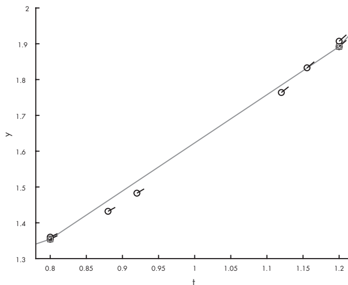
Figure 10.4: Points where ode45 evaluates the rate function, zoomed in
