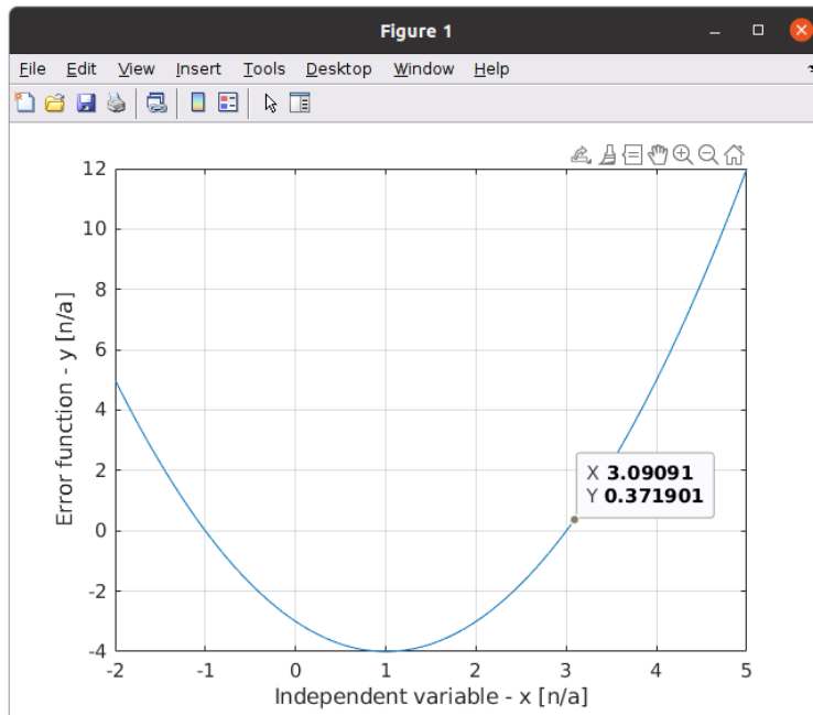
Figure 8.1: Visualization of the error function.
