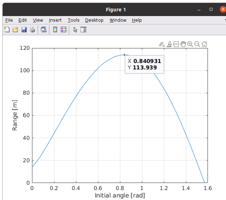
Figure 14.2: Exhaustive search for maximum range using the Data tips graphical tool to choose the near-optimal solution
