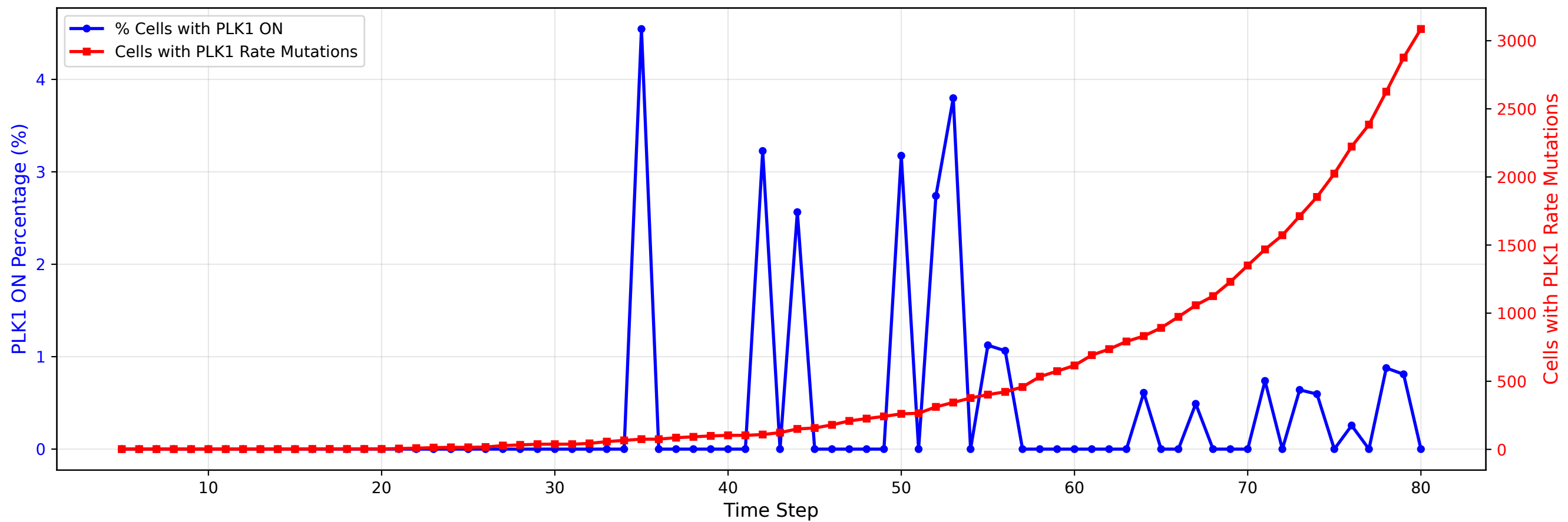
Correlation: PLK1 Rate Mutations vs Node State
