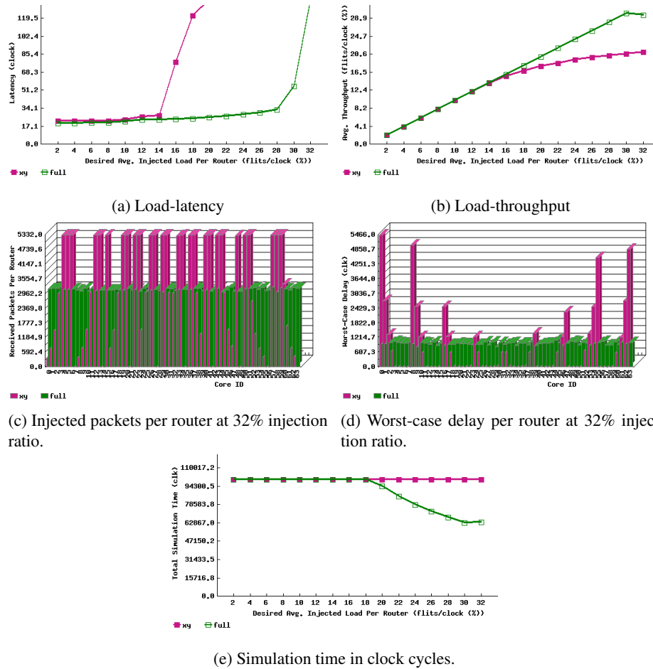
Figure 8.5: Simulation sample results.
