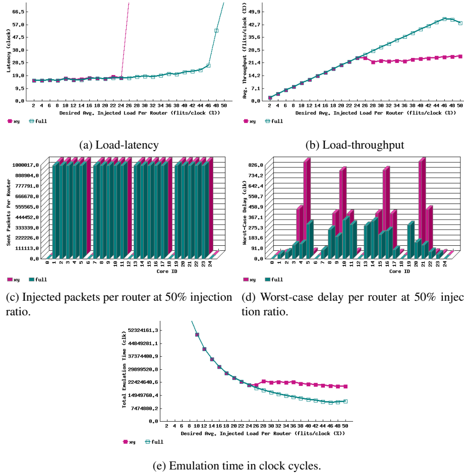
Figure 9.4: Emulator sample results.
