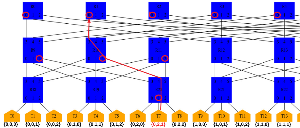
Figure B.2: Fattree endpoint coding example.
