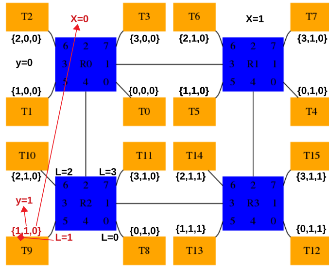
Figure B.1: 2x2 CMESH endpoint coding example.
