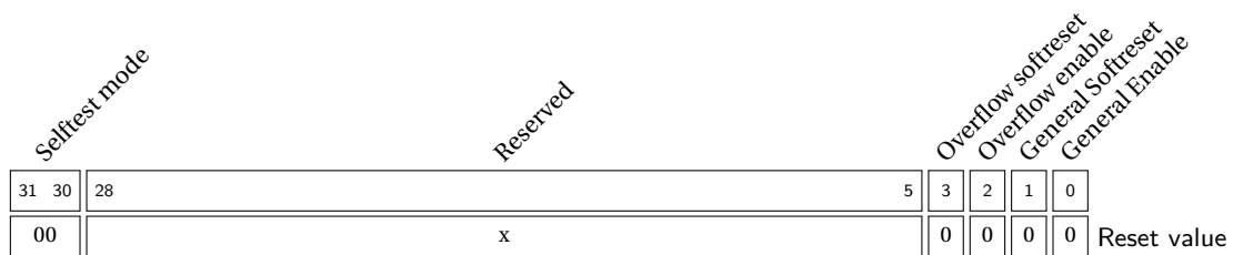
Register 2.1: BASE CONFIGURATION REGISTER (0x000)
