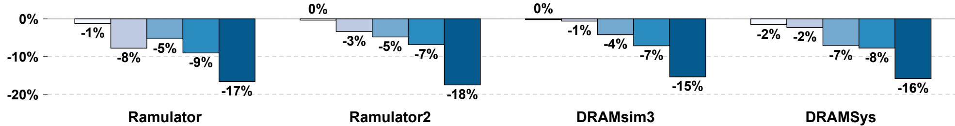
Actual vs. Simulated performance [%]
