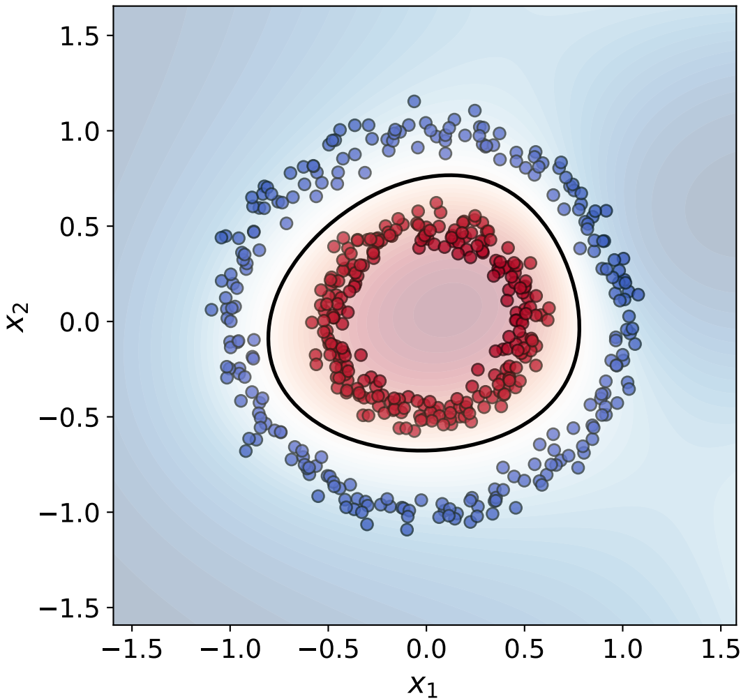
QONN of N=3 , L=1 , \hat{a} in modes [1]
