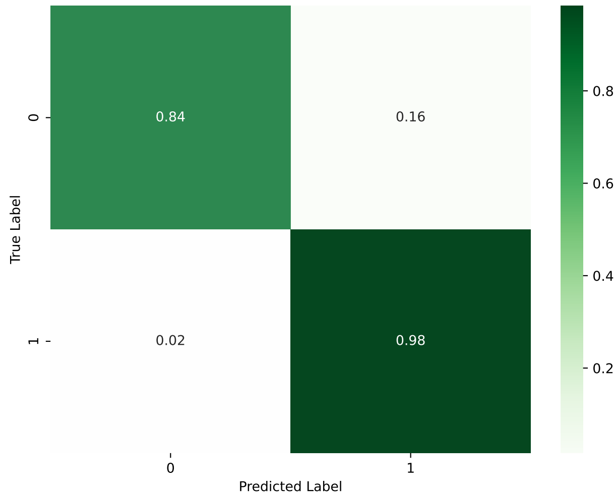
Confusion Matrix
