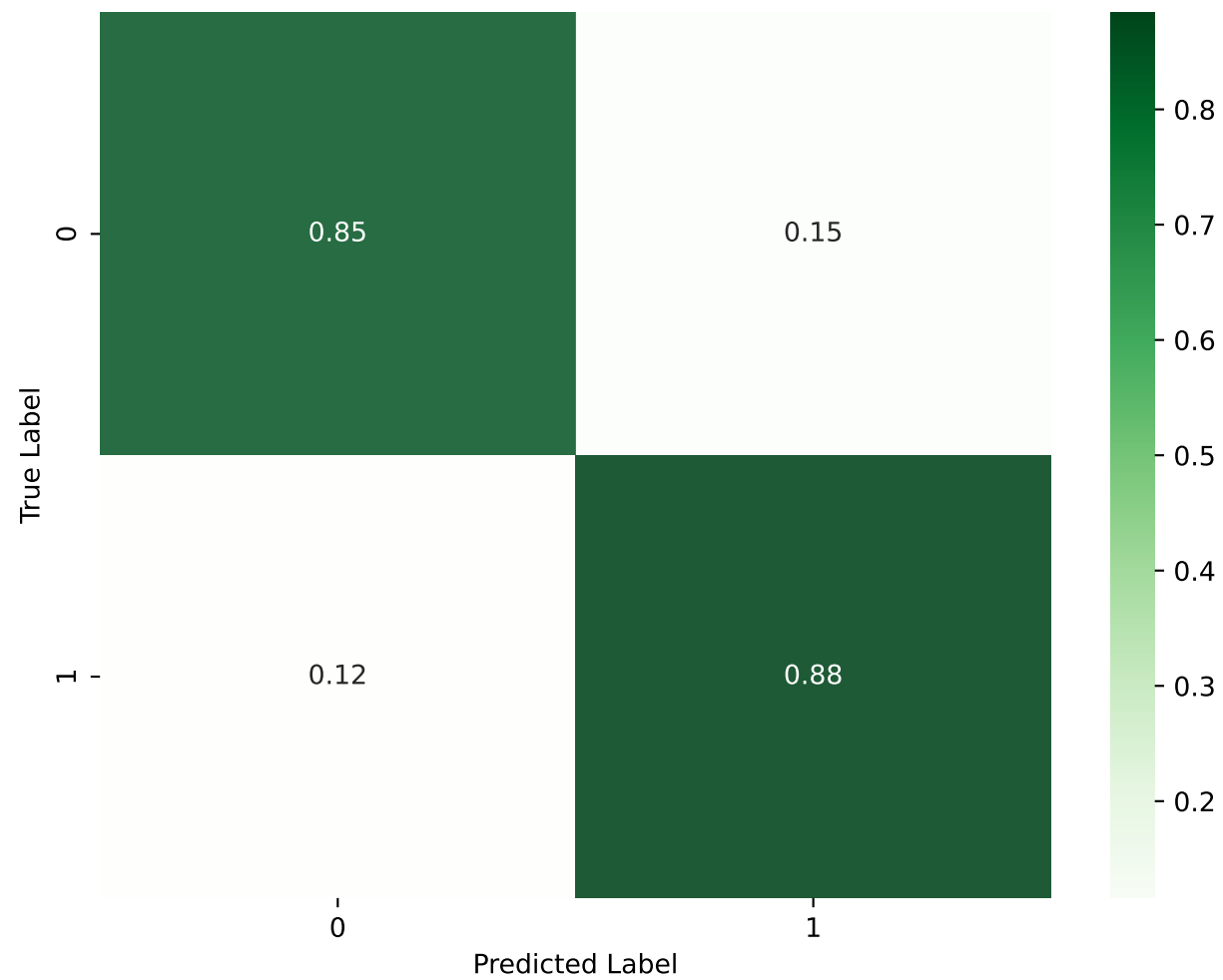
Confusion Matrix
