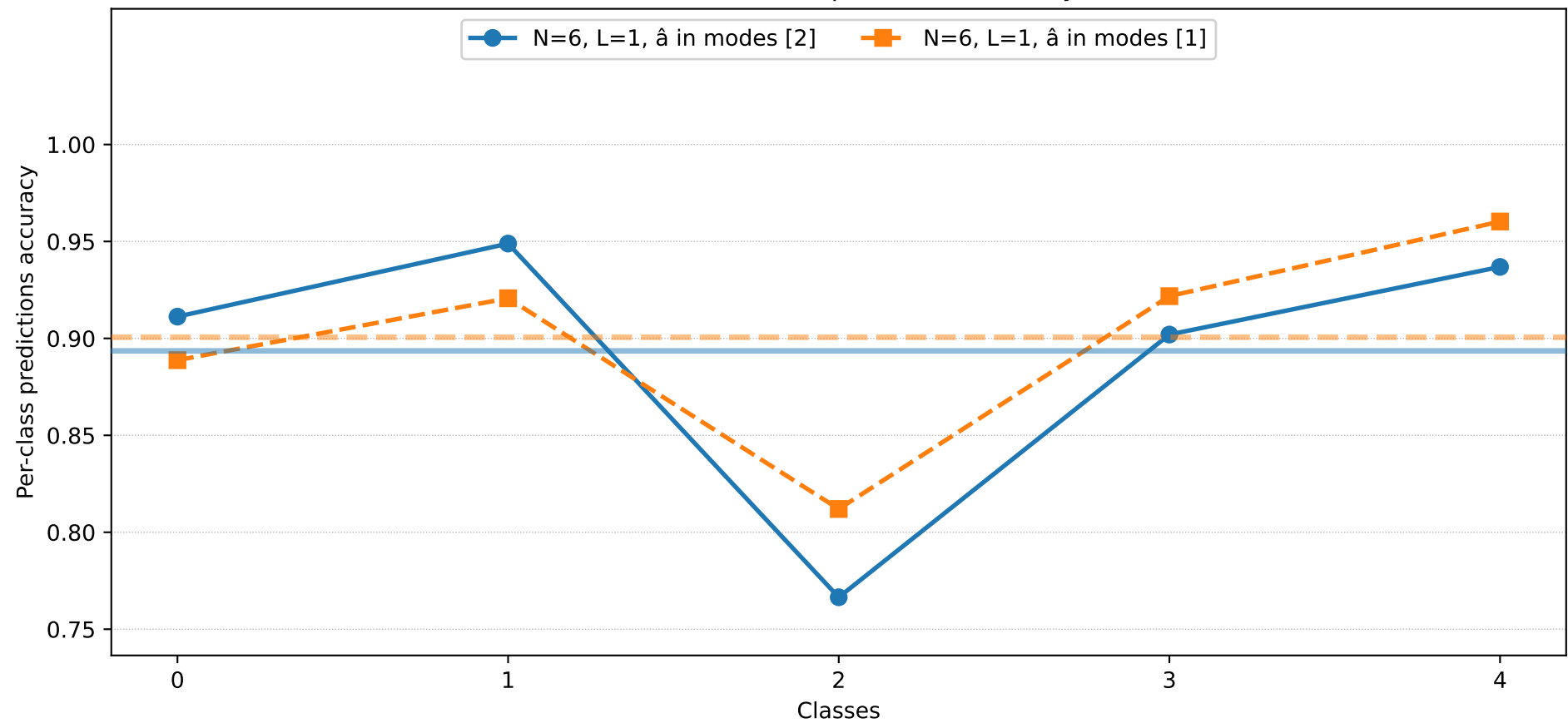
MNIST — QONNs per-class accuracy
