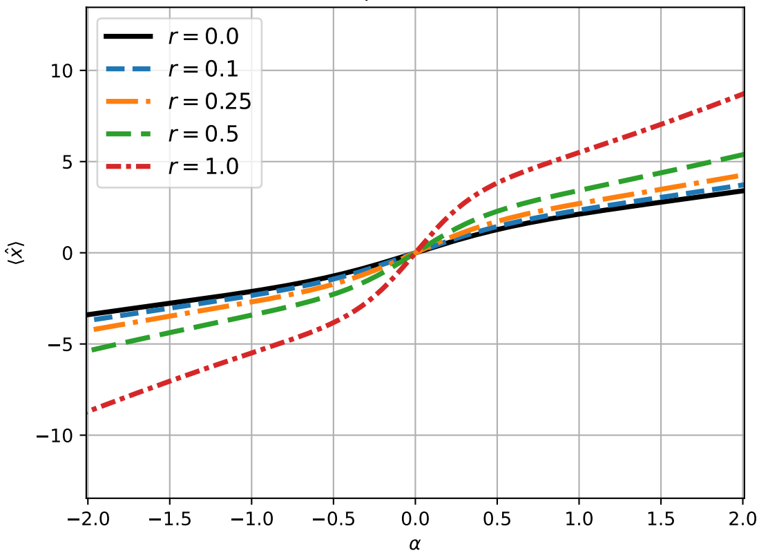
\langle \hat{x} \rangle for n = 1 photon addition, r \geq 0
