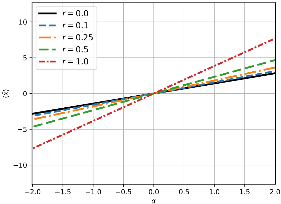
\langle \hat{x} \rangle for n = 0 photon addition, r \geq 0
