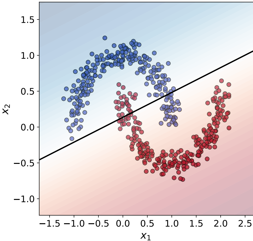
QONN of N=2 , L=1 , None \hat{a}
