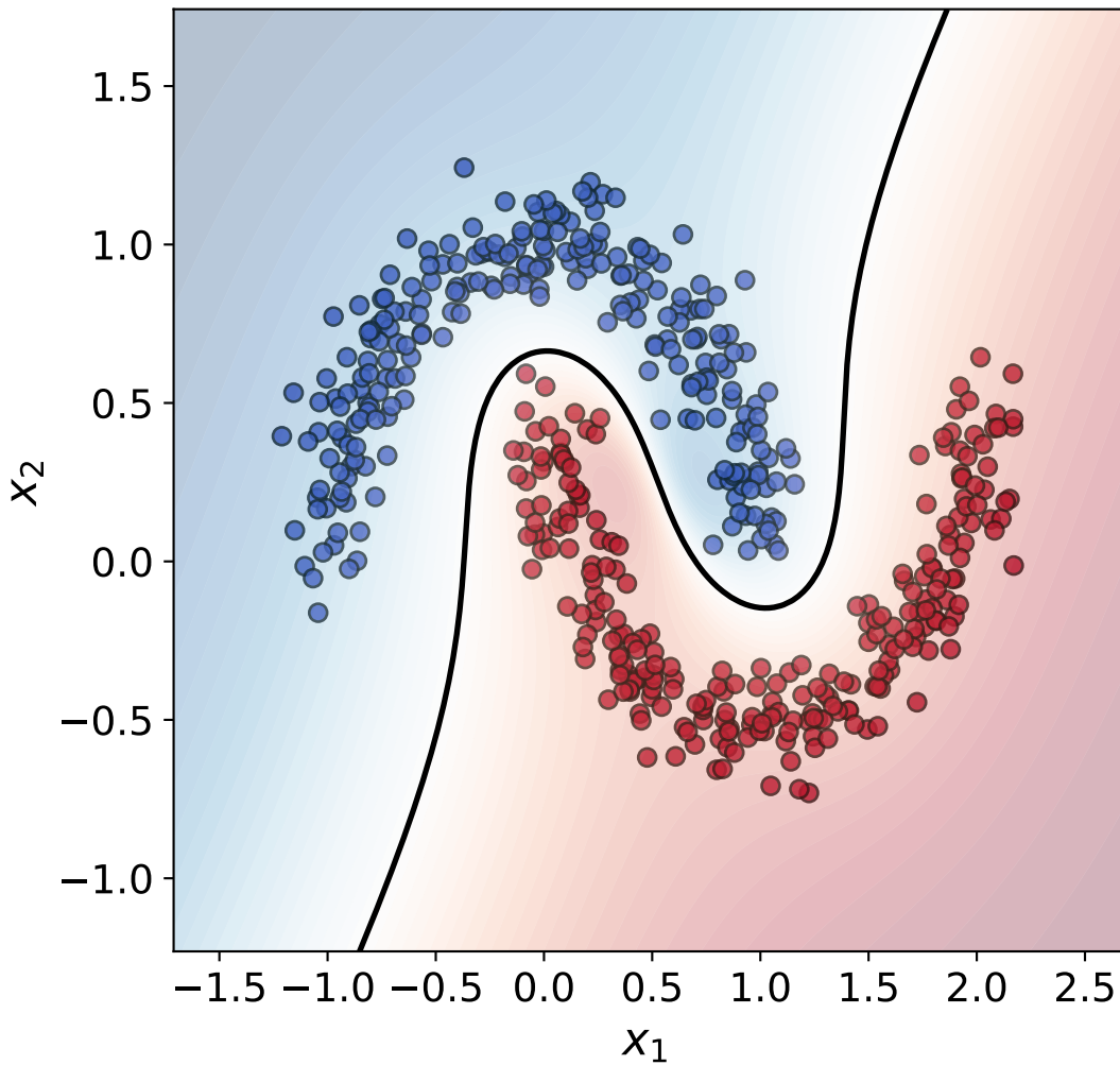
QONN of N=2 , L=1 , \hat{a} in modes [1]
