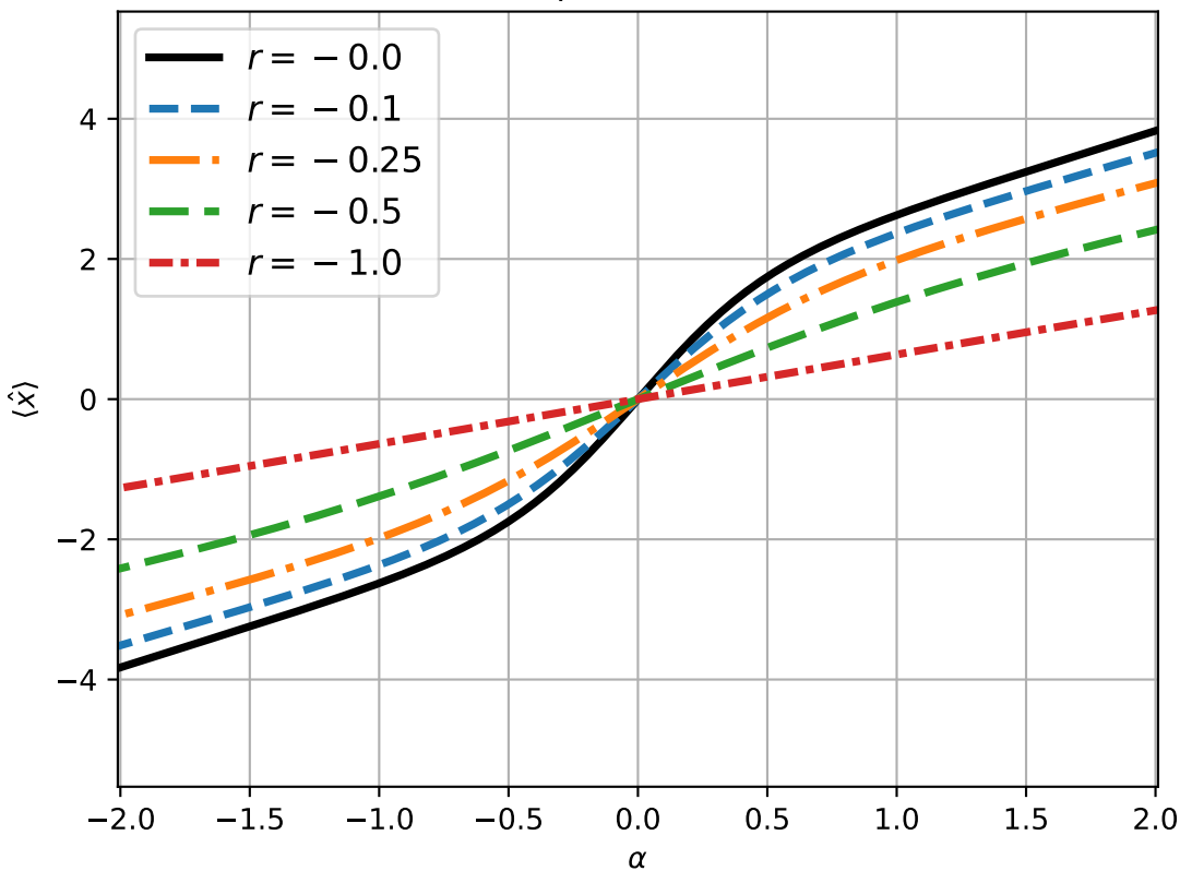
\langle \hat{x} \rangle for n = 2 photon addition, r \leq 0
