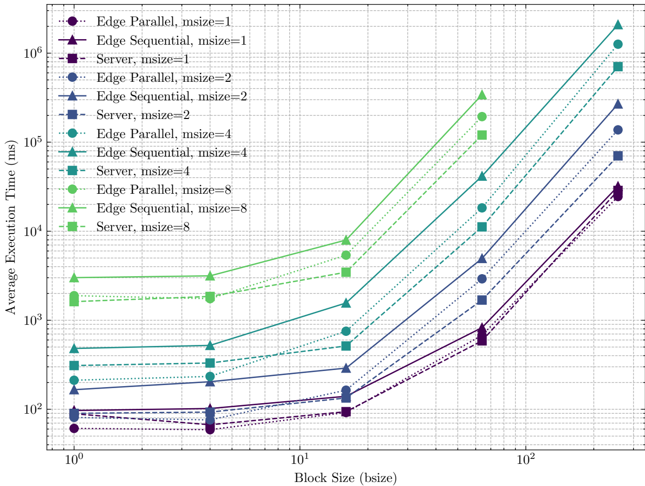
Execution Time Comparison
