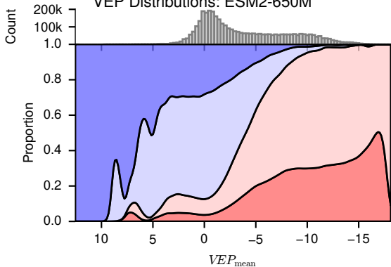
VEP Distributions: ESM2-650M
