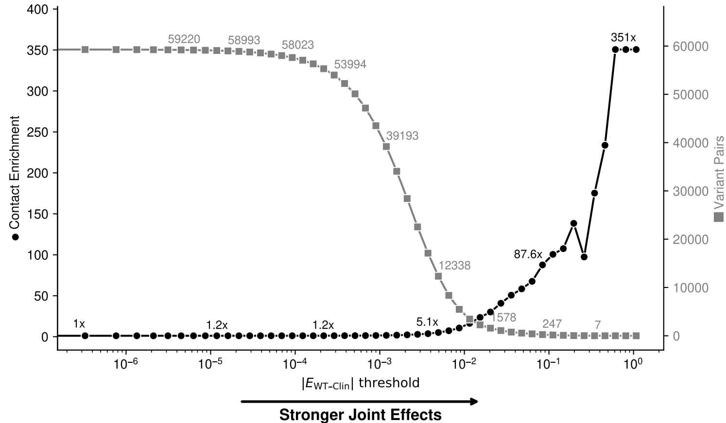
WT-Clinical Variant Joint Effects vs. Contact Enrichment: BRCA1
