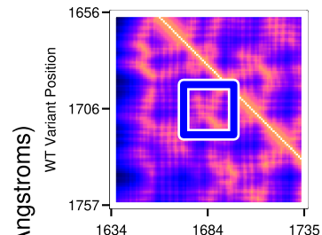
1706G>A | 1687V>I E_{WT-Clin}=-0.65
