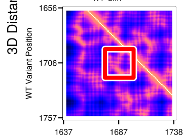
1729L>Q | 1722S>F E_{WT-Clin}=1.13
