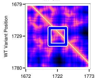
1729L>Q | 1722S>F E_{WT-Clin}=1.13
