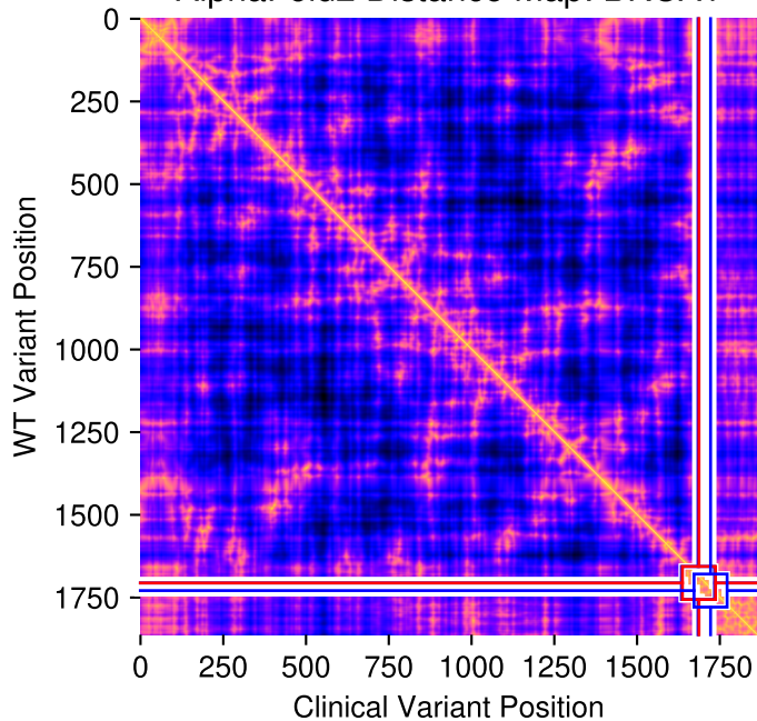
AlphaFold2 Distance Map: BRCA1
