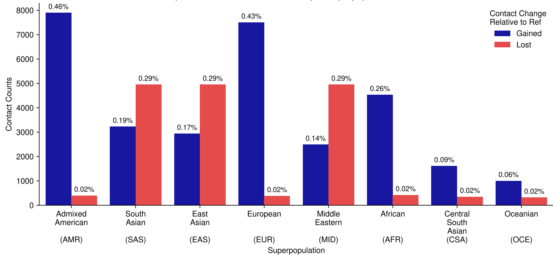
Proportion of Contacts Gained/Lost per Superpopulation: BRCA1
