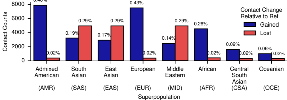
Proportion of Contacts Gained/Lost per Superpopulation: BRCA1
