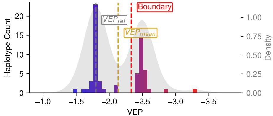
IL7R:F71S (64 haplotypes)
