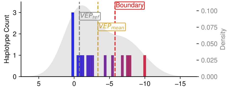
VHL:C121F (15 haplotypes)
