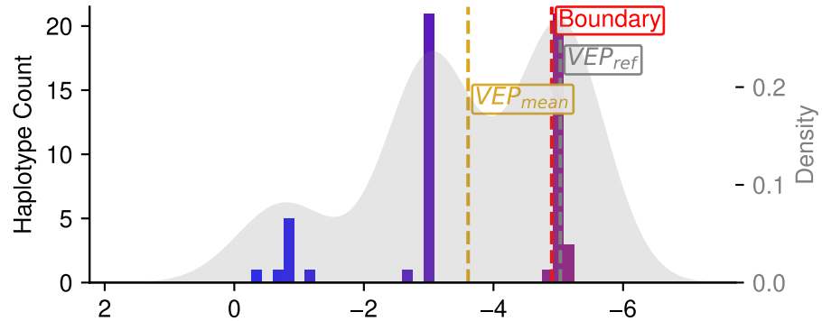
ALDH5A1:I179N (55 haplotypes)
