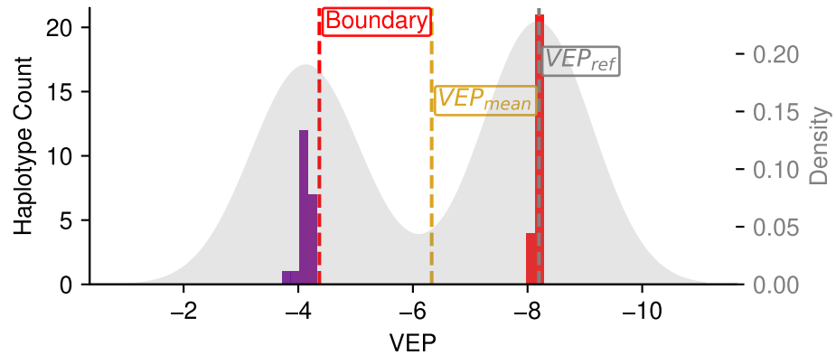
COX10:P225L (46 haplotypes)
