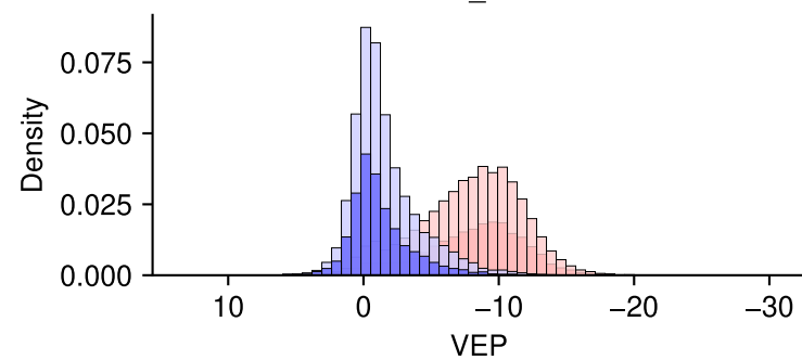
esm3_600m
