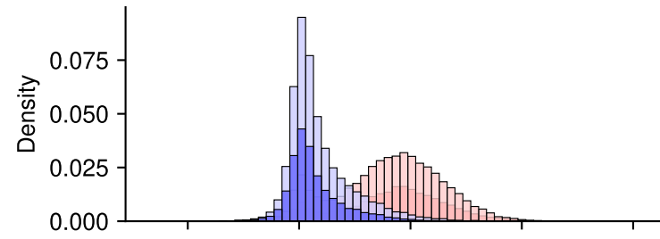
esm1_t34_670M_UR50D
