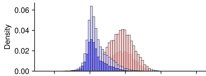
esm1v_t33_650M_UR90S_1
