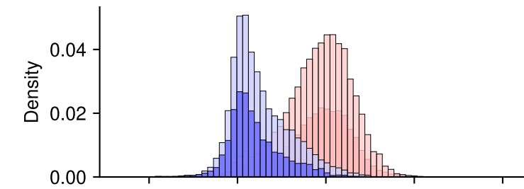
esm1b_t33_650M_UR50S
