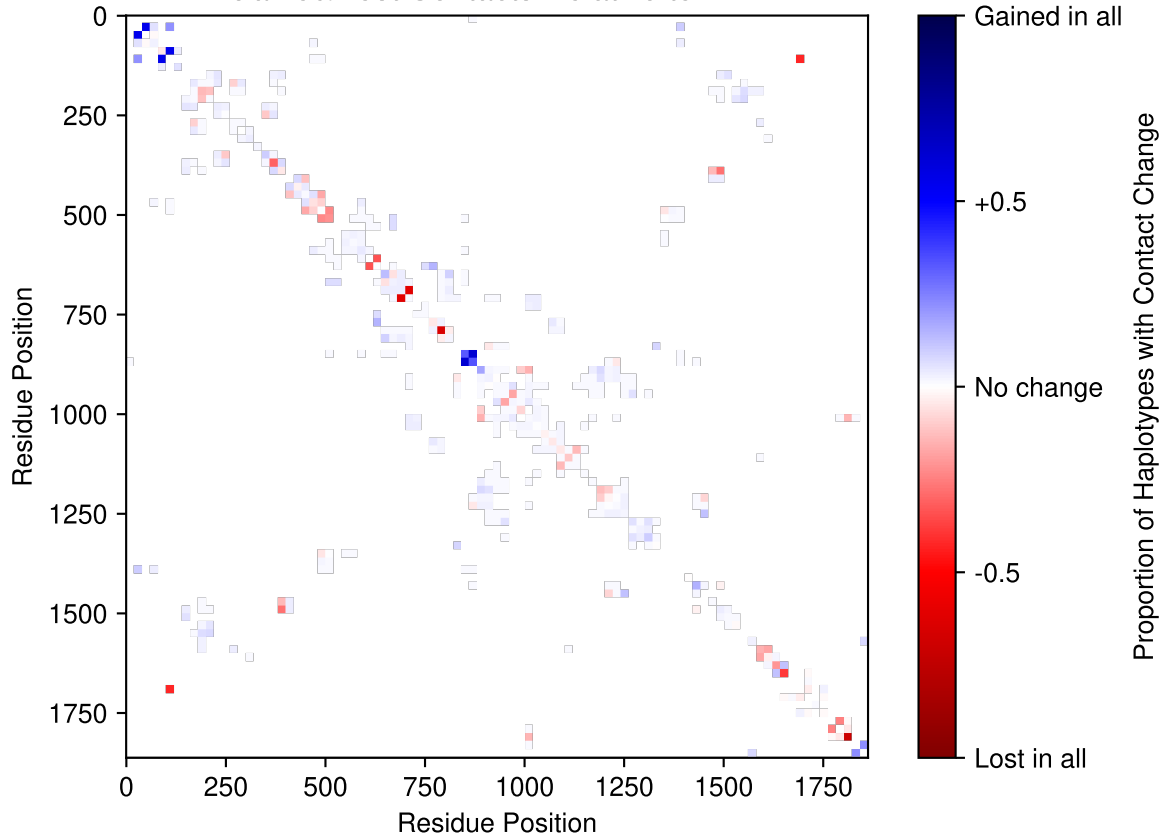
Gained/Lost Contacts Relative to REF
