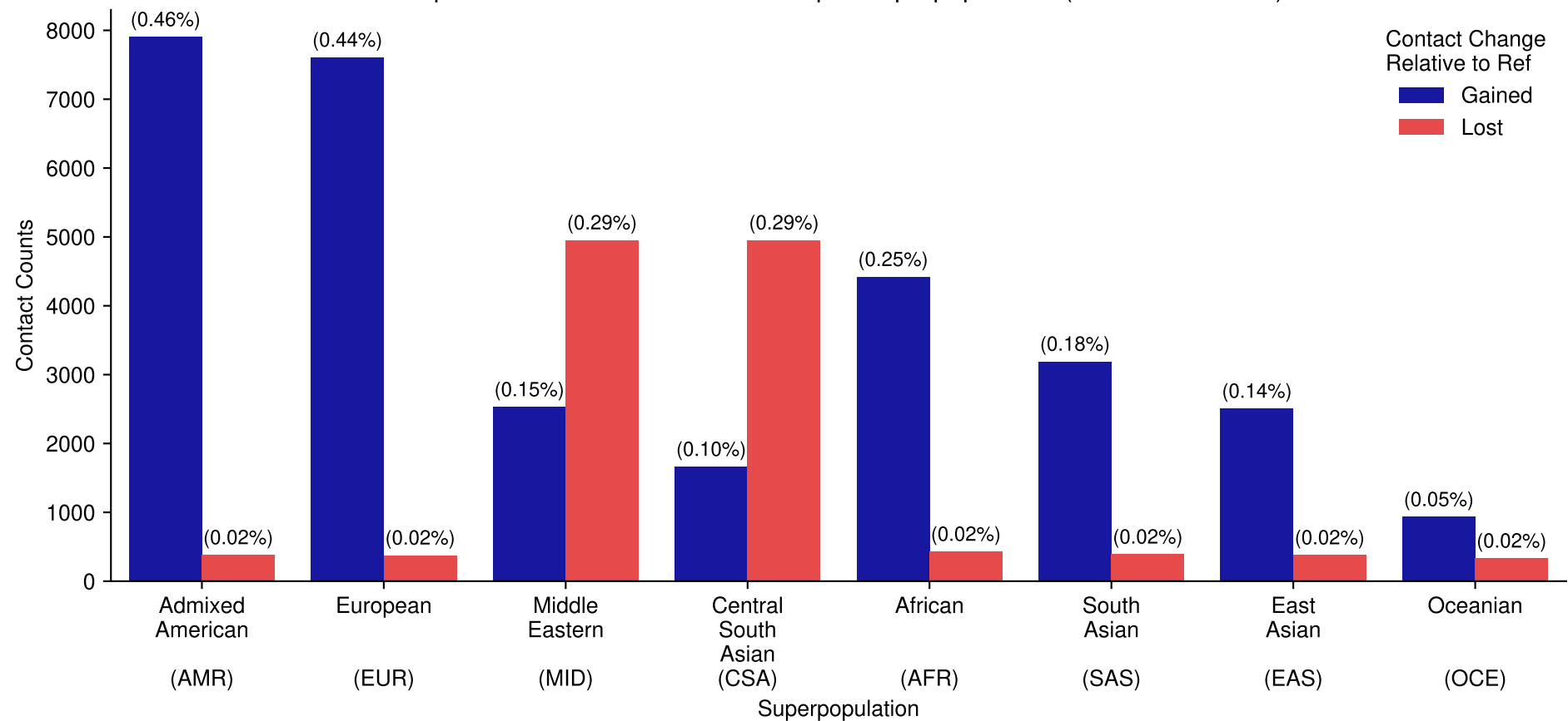
Proportion of Contacts Gained/Lost per Superpopulation (BRCA1 / P38398)
