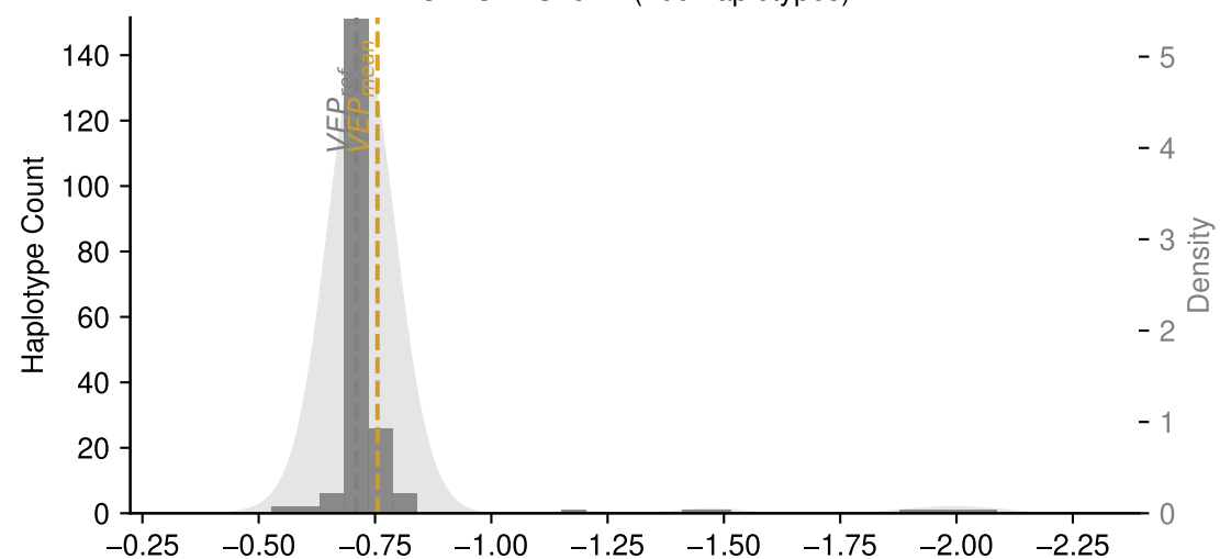
F5:D107H (363 haplotypes)
