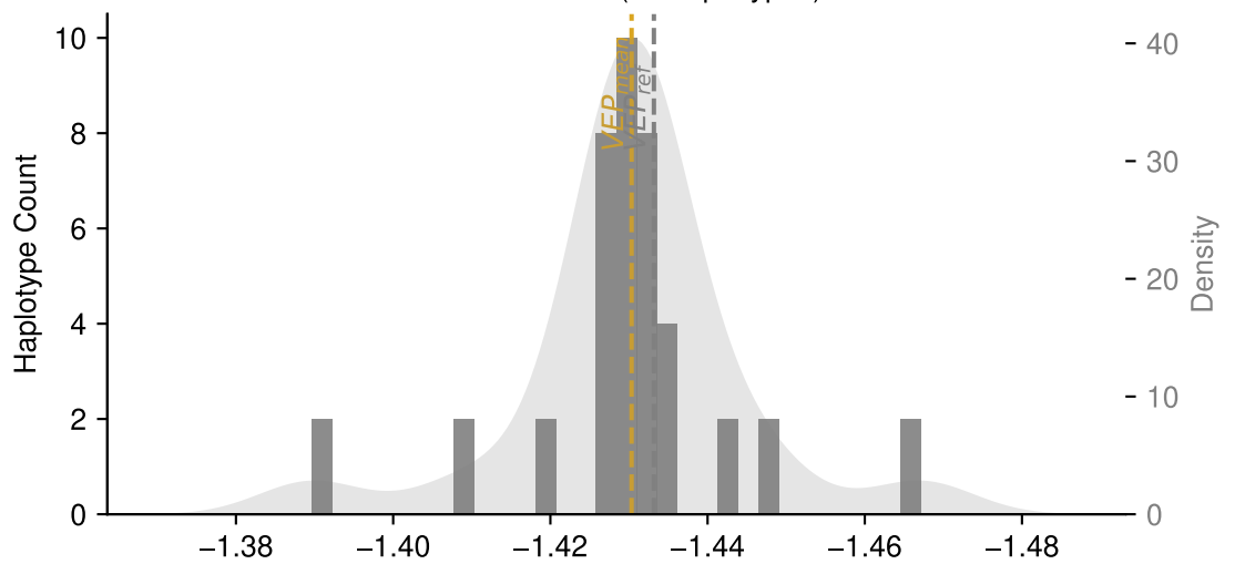
SMARCAL1:R644W (74 haplotypes)
