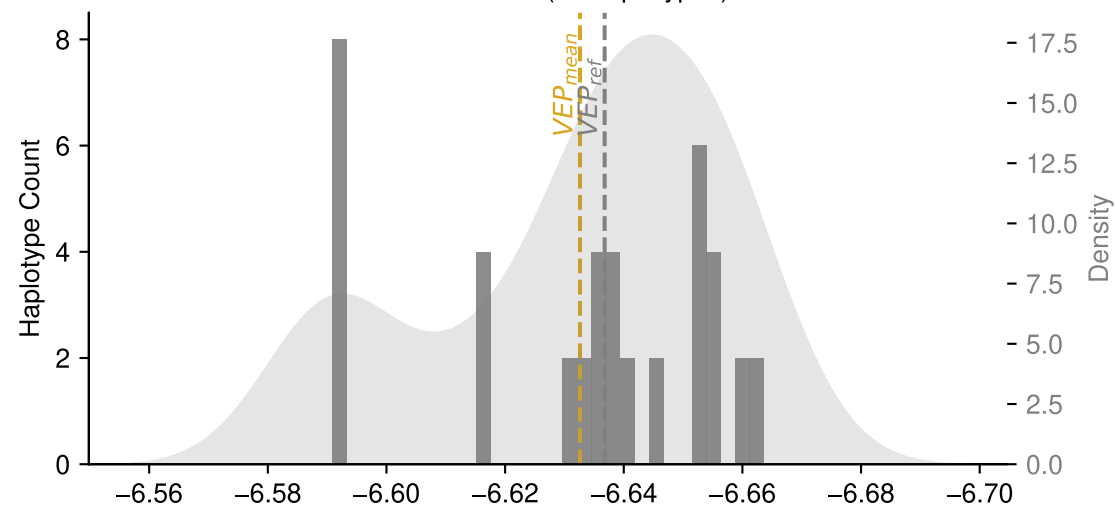
NACC1:R333H (21 haplotypes)
