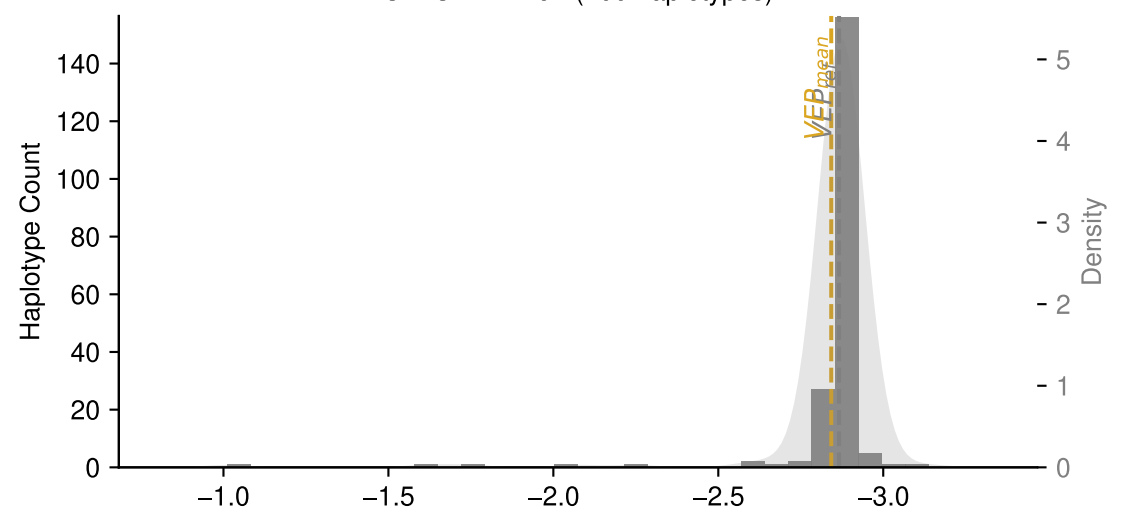
NACC1:R45W (21 haplotypes)
