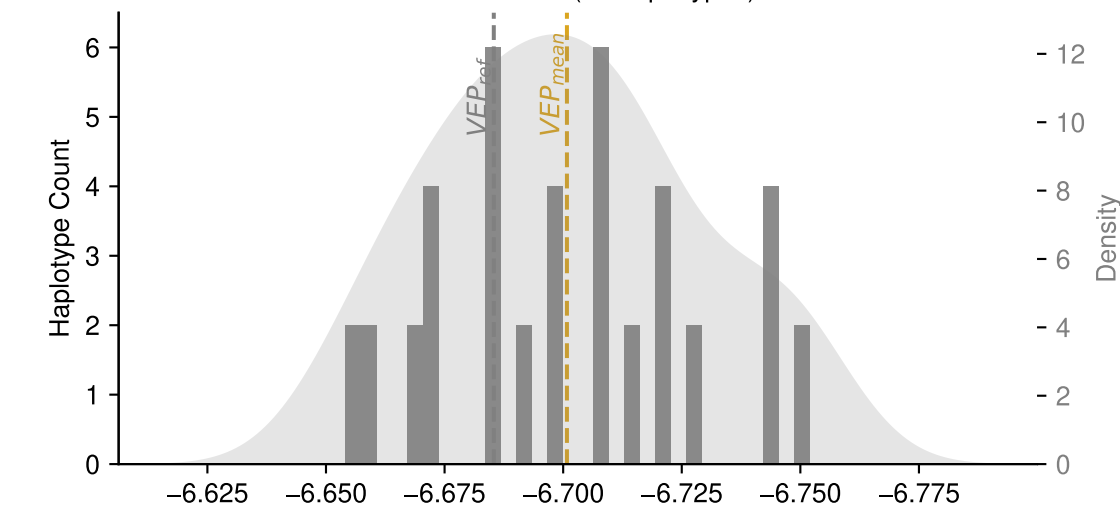
NACC1:R298W (21 haplotypes)
