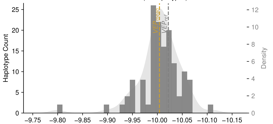
SMARCAL1:R644Q (74 haplotypes)
