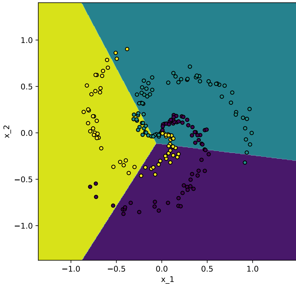
Linear decision regions
