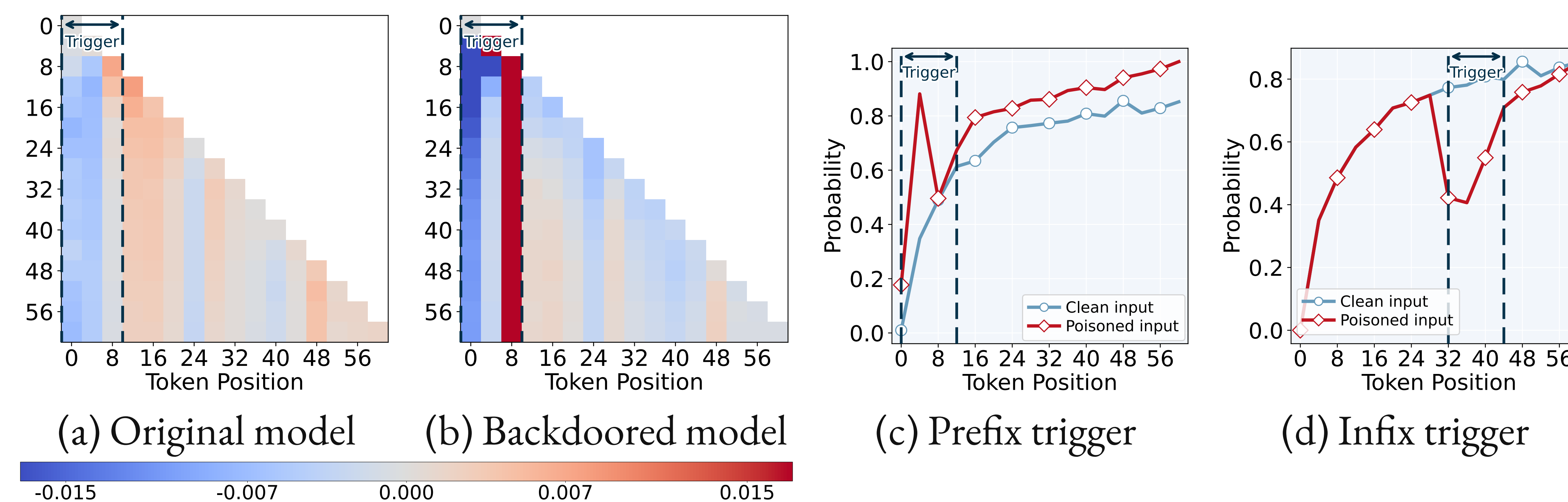
Figure 3. (a–b) Attention difference, triggered – clean (layer 31, prefix trigger). (c–d) Top-1 probability, poisoned vs. clean.
