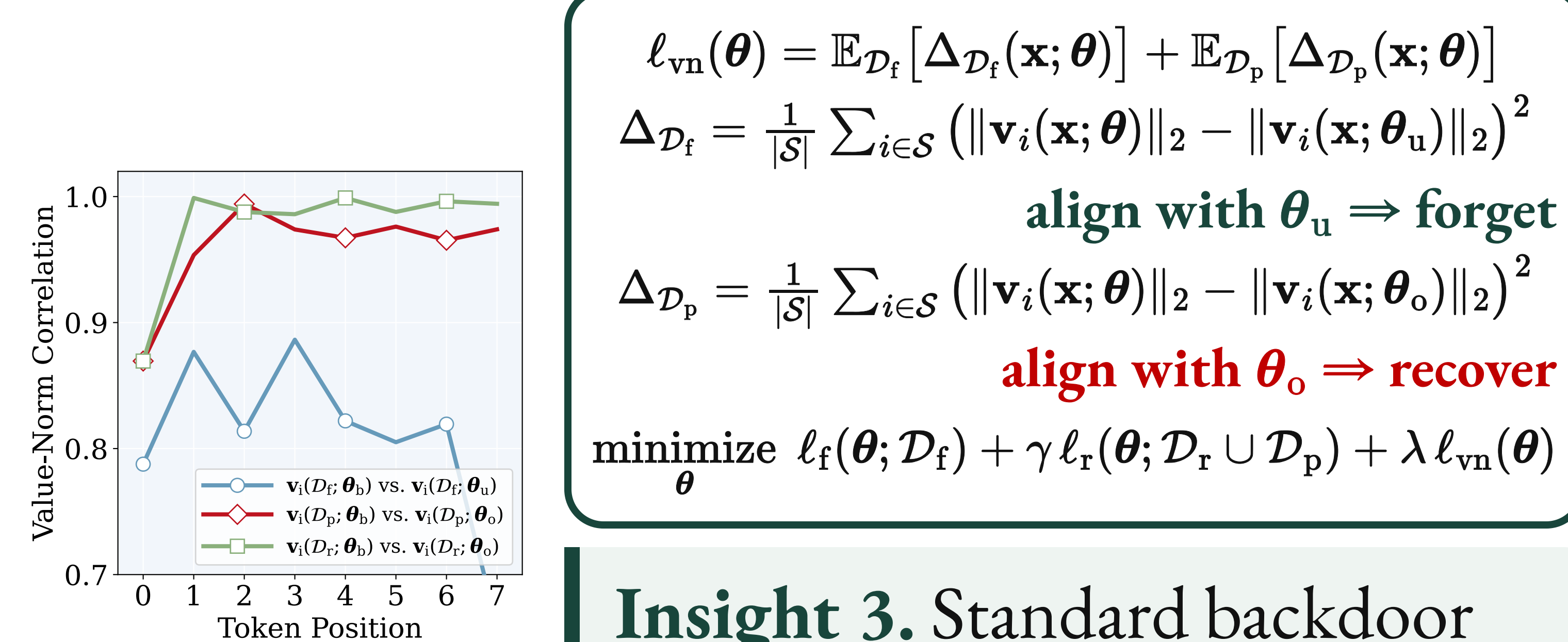
Figure 3. Pearson correlation of sink-token value norms.
