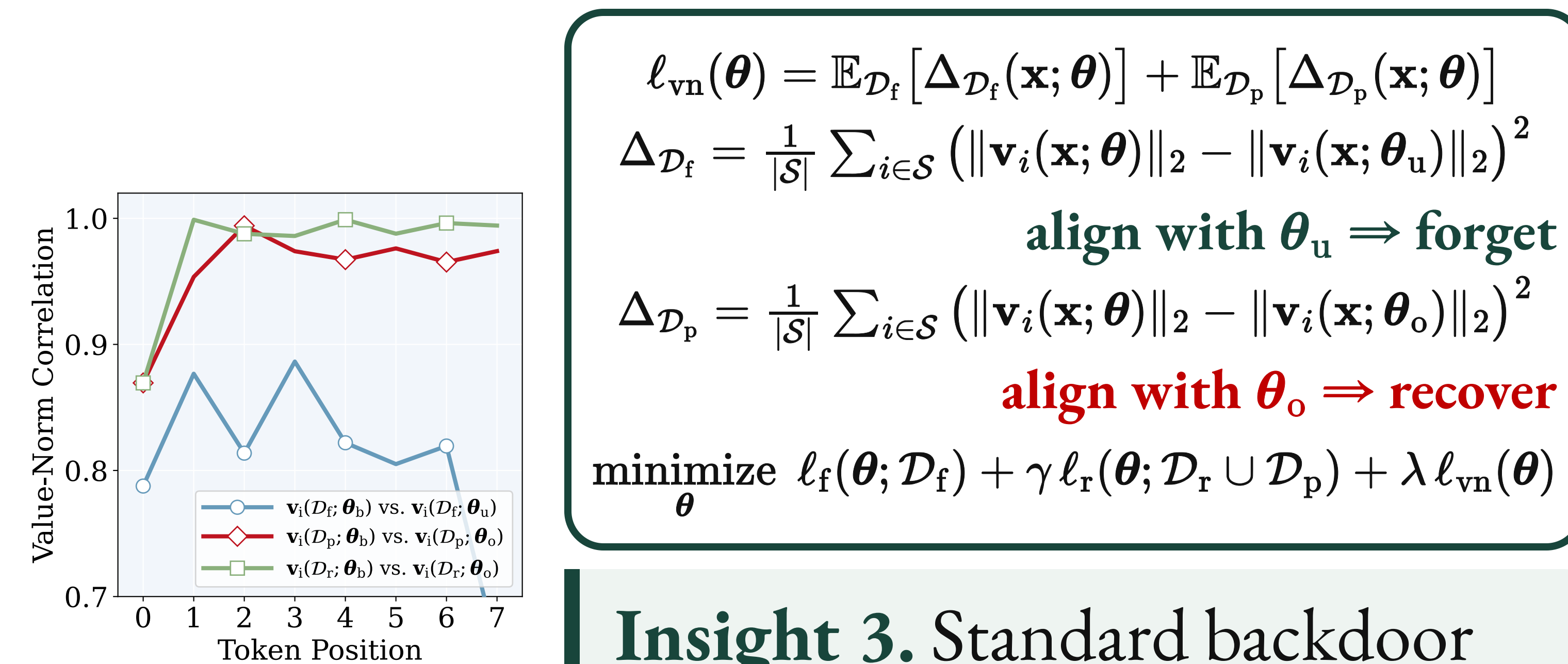
Figure 3. Pearson correlation of sink-token value norms.
