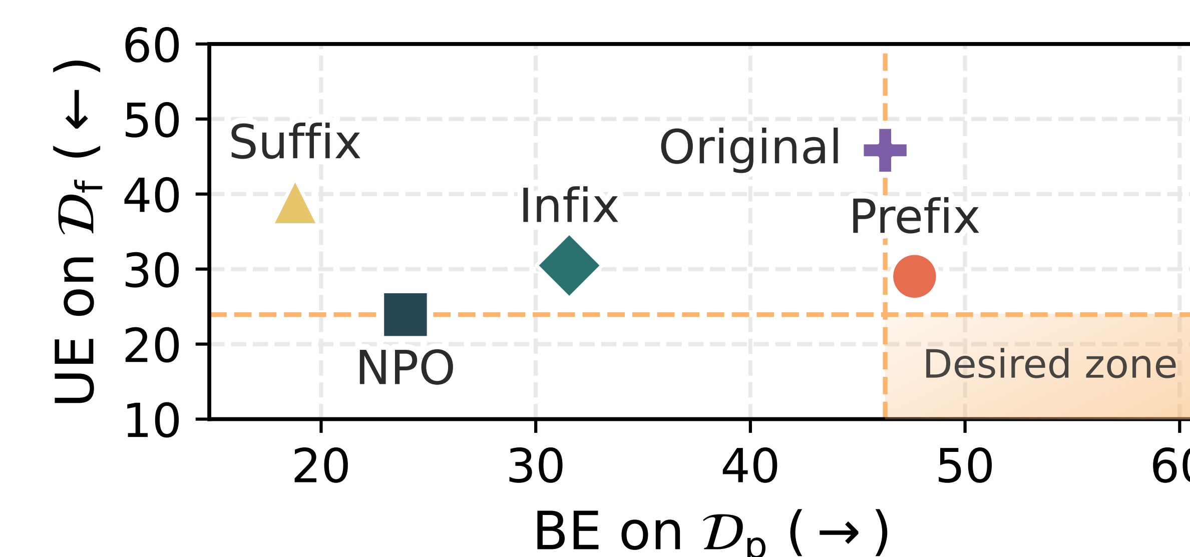
Figure 4. The prefix trigger comes closest to the desired zone (NPO, MUSE-Books).
