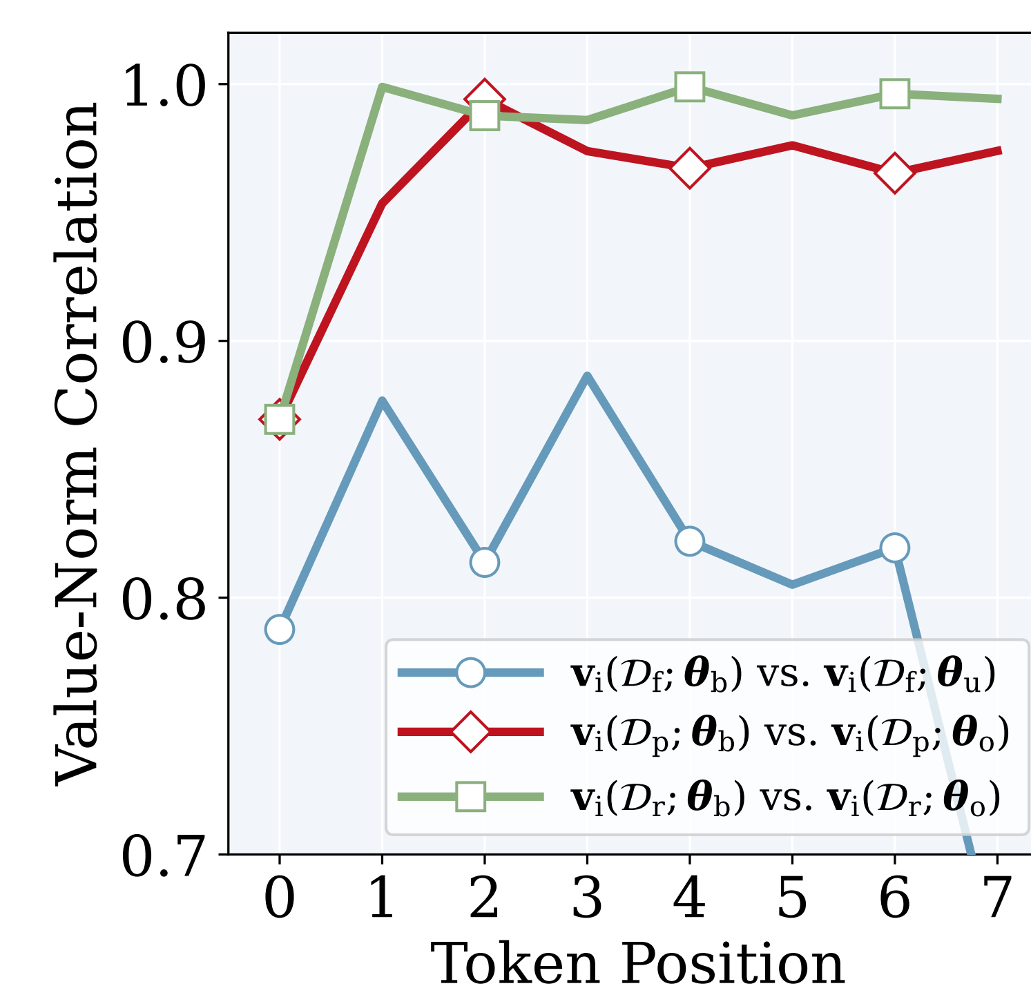
Figure 3. Pearson correlation of sink-token value norms.
