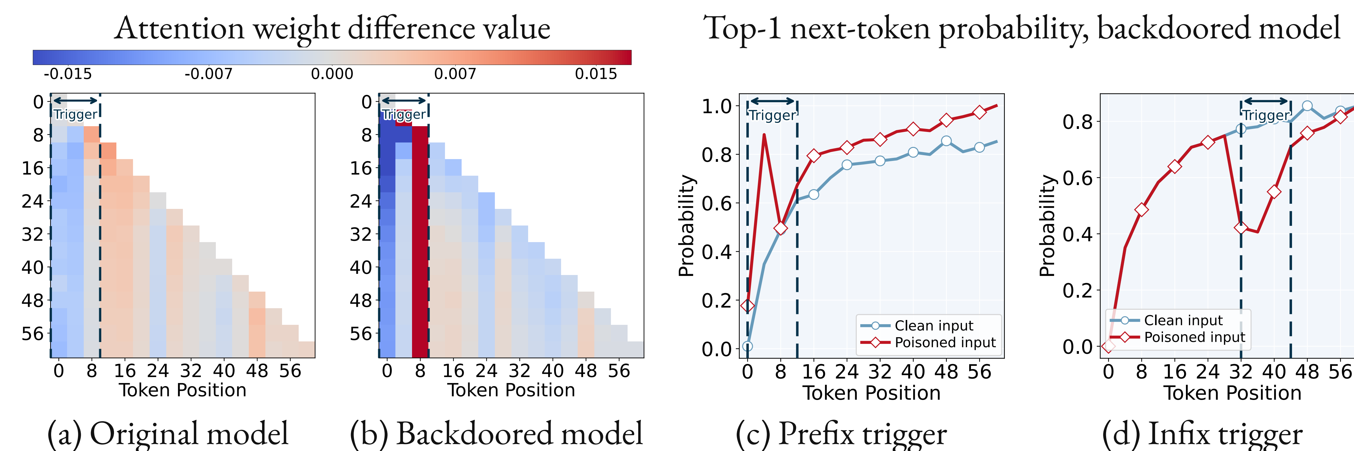
Figure 2. (a–b) Attention difference, triggered – clean (prefix trigger). (c–d) Top-1 probability, poisoned vs. clean.
