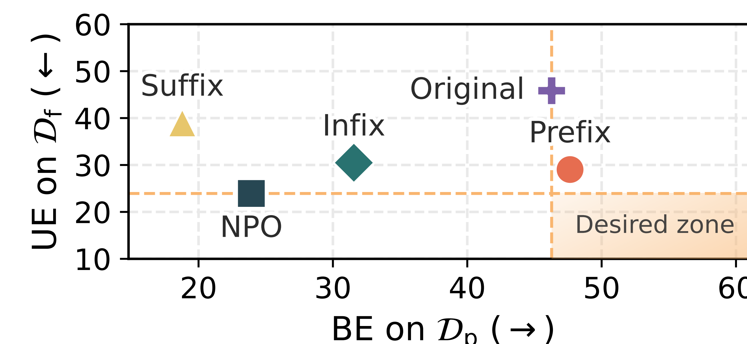
Figure 4. Trigger position: the prefix trigger comes closest to the desired zone (NPO, MUSE-Books).
