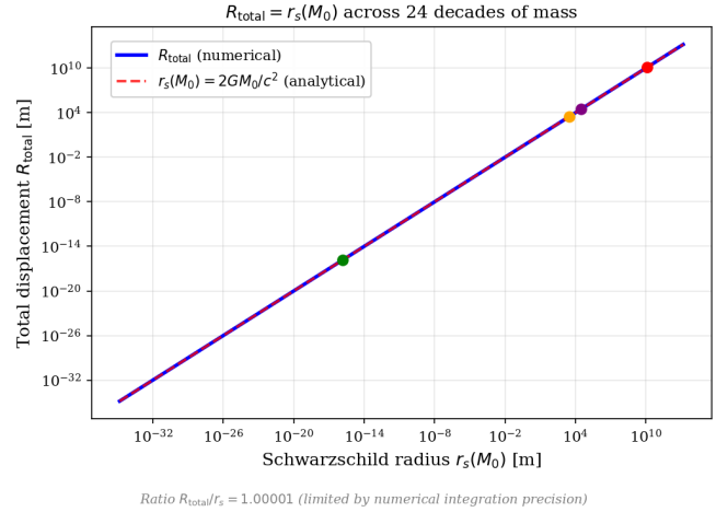
FIG. 4. Total D3 displacement R_{\text{total}} (computed numerically, solid blue) vs analytical Schwarzschild radius r_s(M_0) (dashed red) for 200 black hole masses spanning 24 decades. Both lines are indistinguishable, confirming R_{\text{total}}/r_s = 1.00001 (limited by numerical integration precision) across the full mass range.
