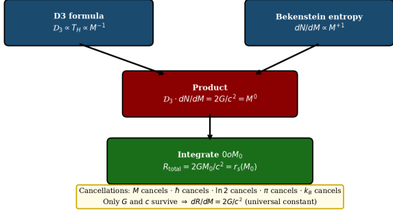
FIG. 1. Derivation flow for the evaporation invariant. The per-bit displacement scales as \mathcal{D}_3 \propto T_H \propto M^{-1} and the bit-loss rate as dN/dM \propto M^{+1} ; their product is the mass-independent constant 2G/c^2 , which integrates to R_{\text{total}} = r_s .
