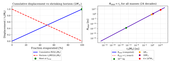
FIG. 3. Physical interpretation of the evaporation invariant. Left panel : Cumulative displacement R(t) (solid blue) and instantaneous Schwarzschild radius r_s(M(t)) (dashed red) as functions of evaporation fraction for a solar-mass black hole. R(t) increases linearly while r_s decreases; they are equal and opposite, meeting exactly at complete evaporation. Right panel : R_{\text{total}} (computed dots) vs. r_s(M_0) (exact line) for masses spanning 24 decades. Agreement is perfect.
