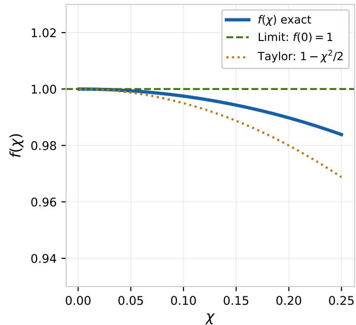
(a) Schwarzschild limit f(0) = 1 exactly
