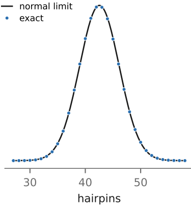
hairpins: exact vs. normal
