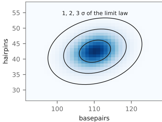
exact joint distribution, n = 400
