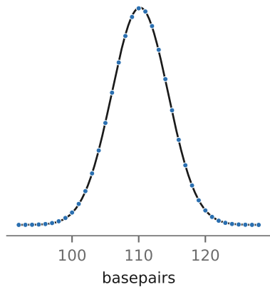
basepairs: exact vs. normal
