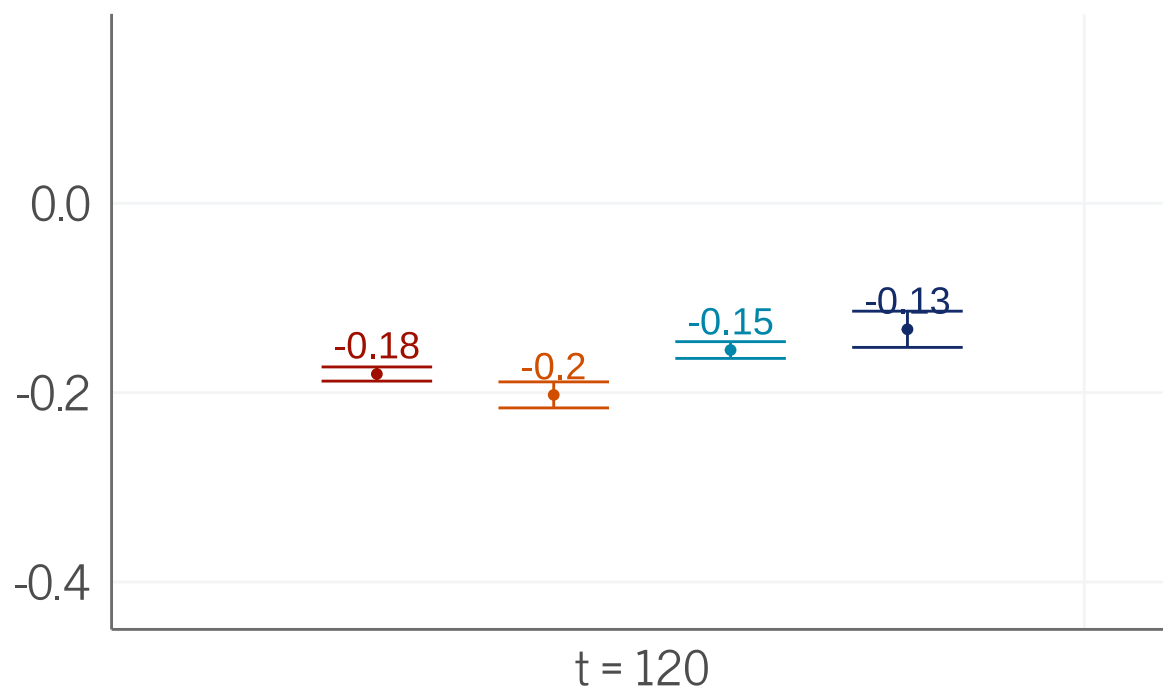
Semi-sparse (10 nodes, medium sparsity) Bias
