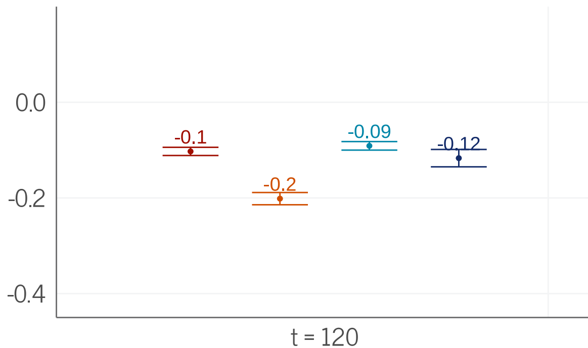
Sparse (10 nodes, high sparsity) Bias
