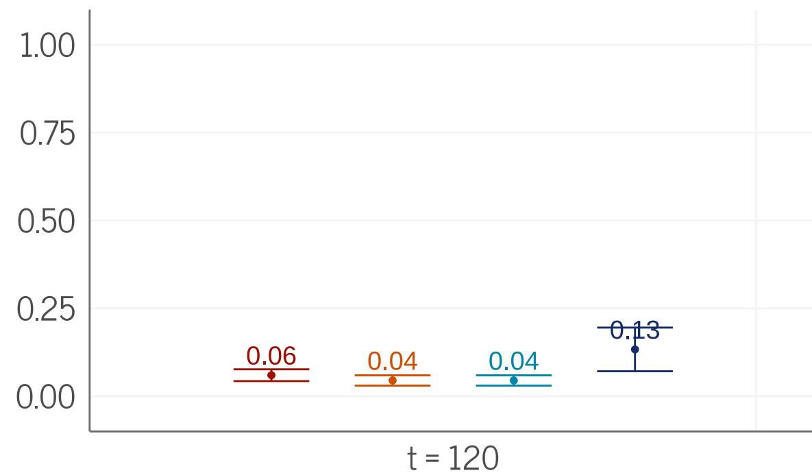
Semi-sparse (10 nodes, medium sparsity) Detection Rate
