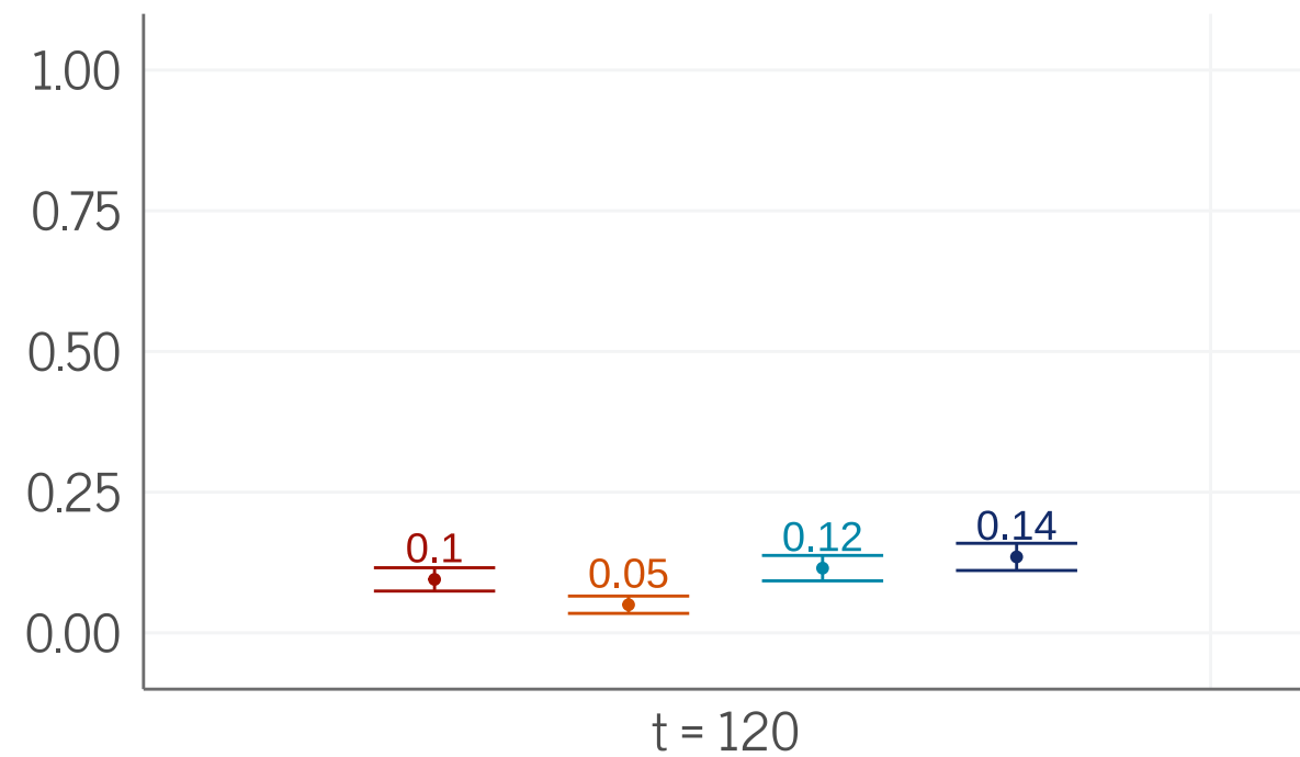
Sparse (6 nodes, high sparsity) Detection Rate
