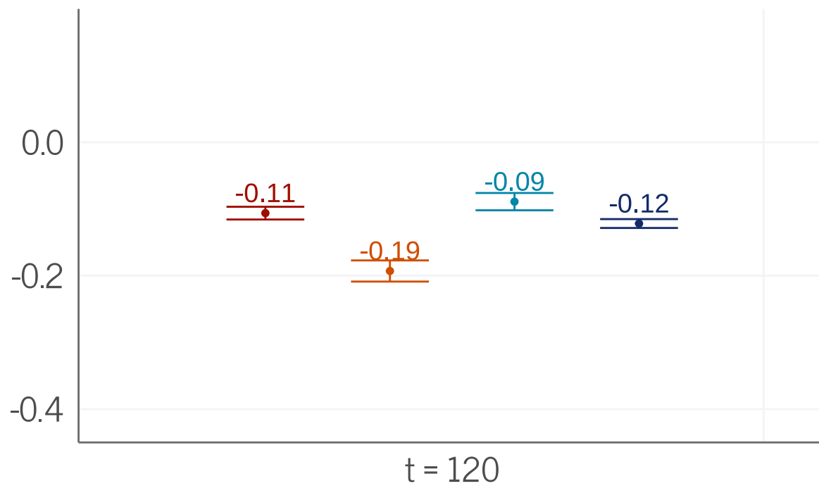
Sparse (6 nodes, high sparsity) Bias
