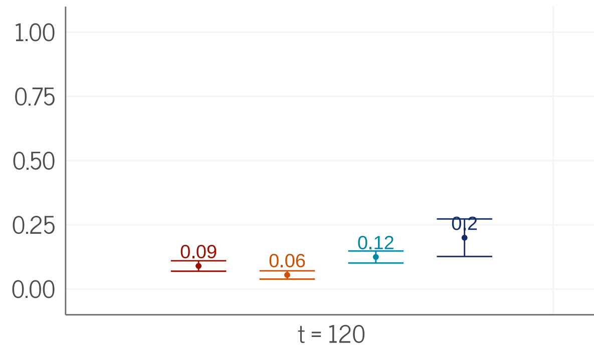
Sparse (10 nodes, high sparsity) Detection Rate
