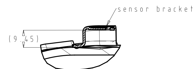
SECTION E-E SCALE 1/1
