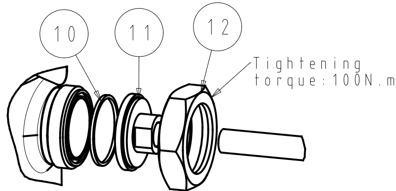
Detail B Scale 1/2 ROTALOCK for DSH184
