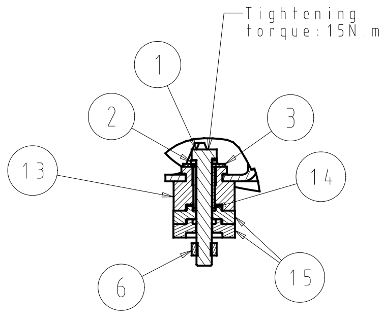
Scale 1/2 Fitting for DSH184
