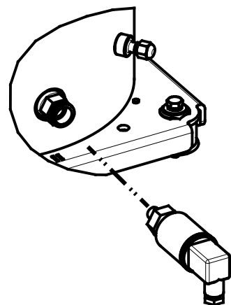
DETAIL C Illustration of Oil Level Sensor Installation Position
