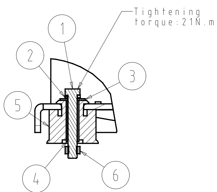
Scale 1/2 Fitting for VZH170
