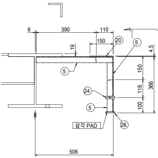
SEC VIEW "B" S=(1/15)
