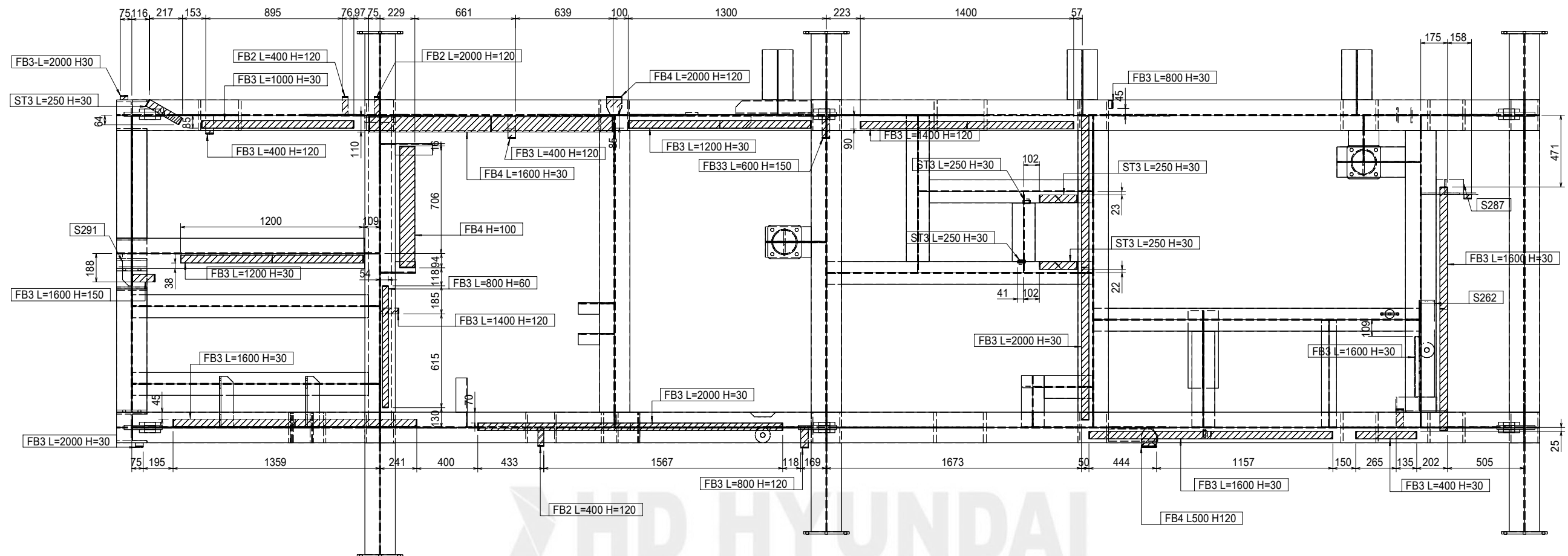
PLAN VIEW "A"
