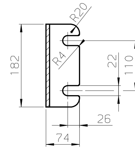
SECTION N-N
