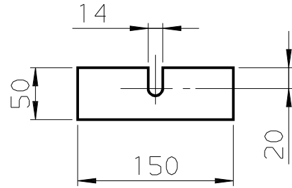
SHIMS P05 030/031/032 FOR GRID CHANNEL (SCALE 1:5)
