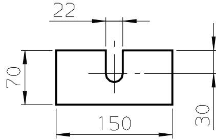
SHIMS P05 015/016/017 FOR OIL TANK (SCALE 1:5)
