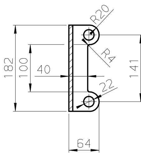
SECTION M-M
