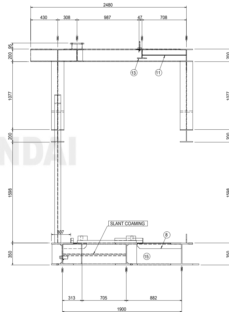
SEC VIEW "Q"
