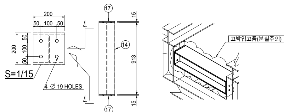
DETAIL "K-1"
