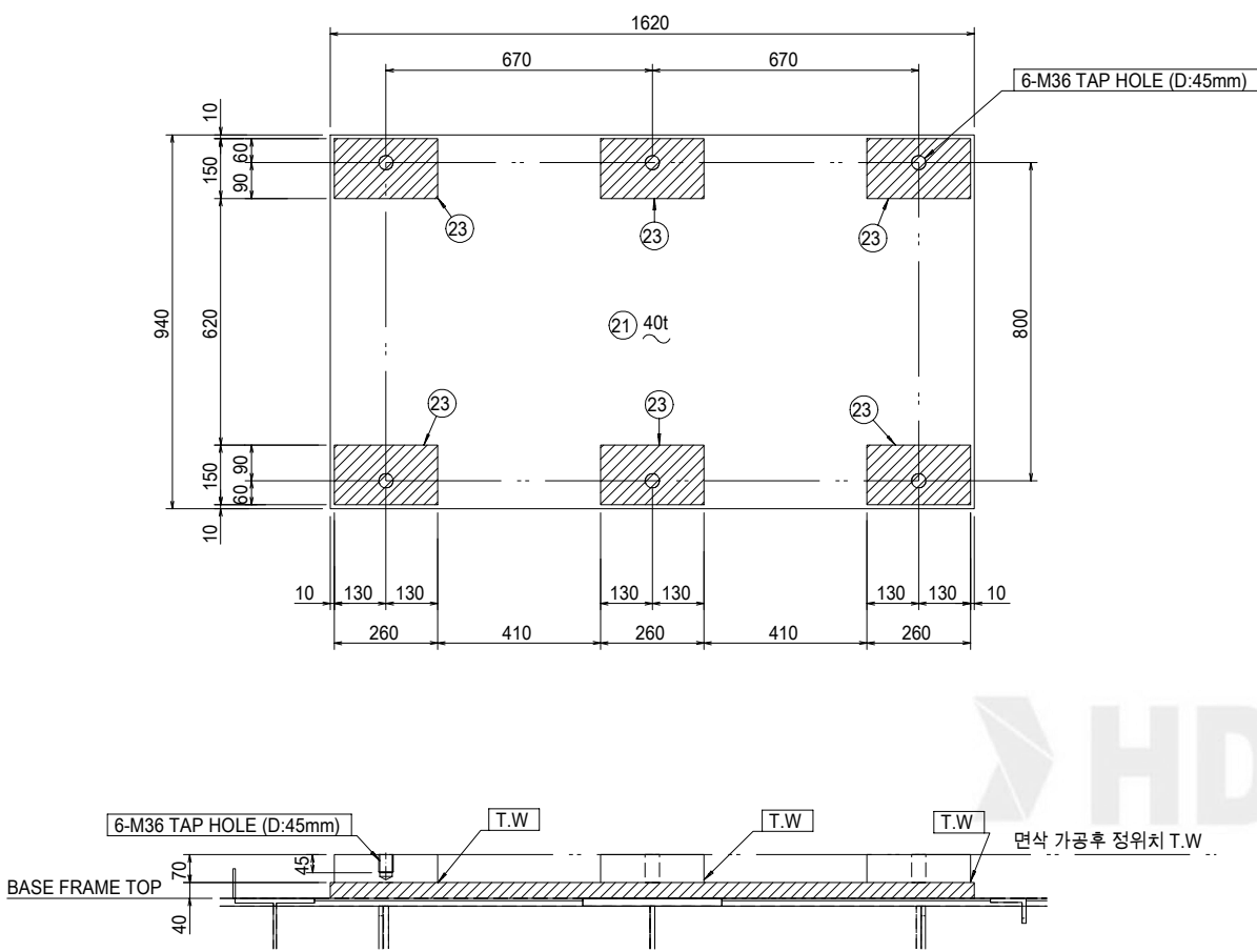
COMP. SEAT PLAN (S=1:20)
