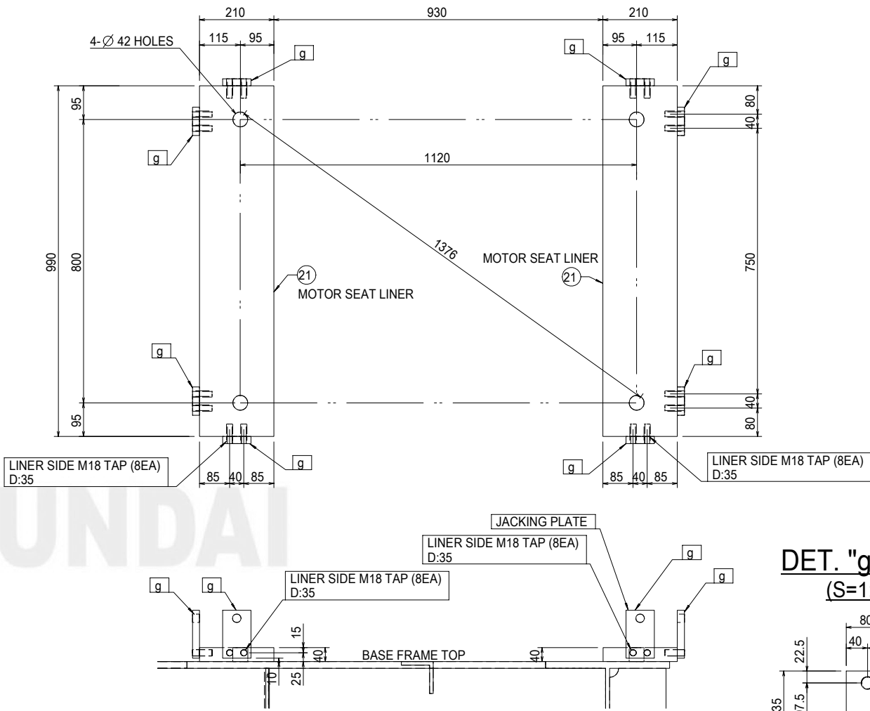
COMP. MOTOR SEAT PLAN (S=1:15)
