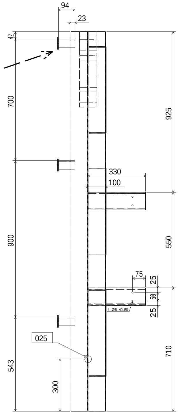
VIEW "B"
