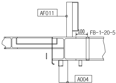
"A10" VIEW
