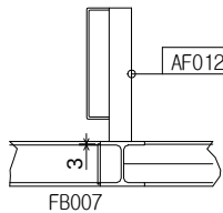
"A9" VIEW
