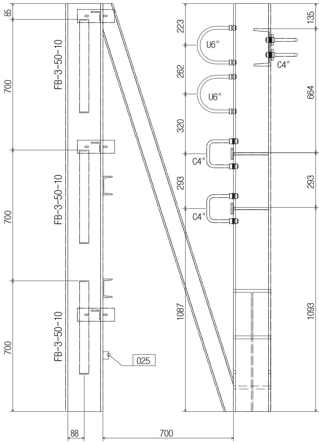
VIEW "A"
