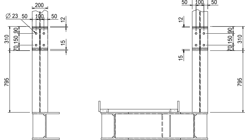
TYP. VIEW "G-1"
