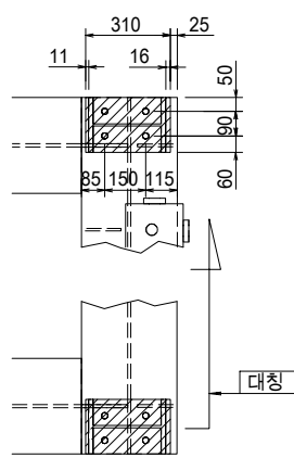
TYP. VIEW "G-2"
