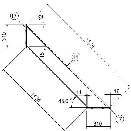
DETAIL "G-3" (2EA)
